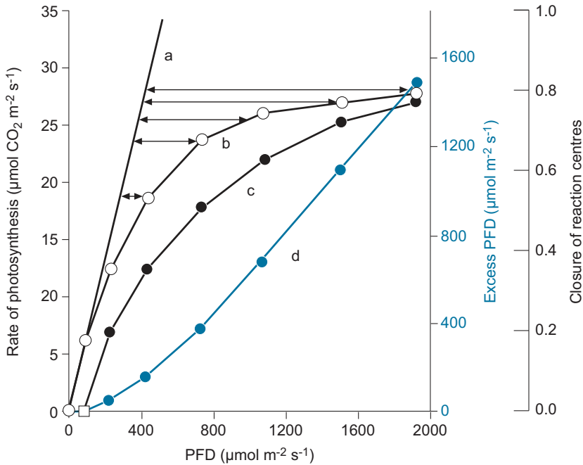
Fig. 3. – Light saturation curve of photosynthesis showing (curve b) the rate of \text{CO}_2 fixation in response to photon flux density, PFD. a) Linear response of photosynthesis with increasing light at low PFD. c) Calculated time of transfer of electrons from PSII including repair of damage by light. d) Excess light energy [3].
