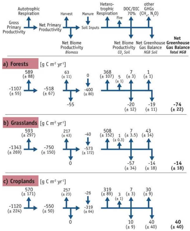
Fig. 6. – \text{CO}_2 fluxes at the ecosystem level, for explanation see text [7,8]. Arrows pointing to the top indicate C fluxes to the atmosphere, while arrows pointing to the bottom indicate C fluxes to the soil or into biomass.
