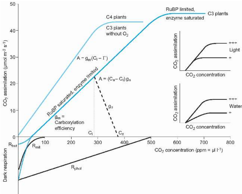
Fig. 4. – Schematic representation of the response of \text{CO}_2 -assimilation in C4 and C3-plants to the \text{CO}_2 concentration in the atmosphere. Positive values represent \text{CO}_2 uptake, negative values represent \text{CO}_2 emission. The inserted figures show that changes in light climate change the saturation point of the \text{CO}_2 -fixation, while limitations in water change the slope of the reaction. For further explanations see text [3].
