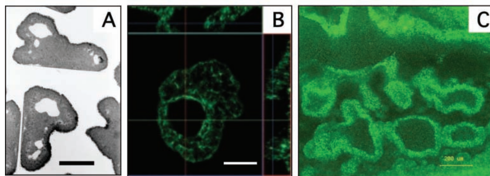
Figure 2. Cross-sections of biofilm colonies produced by (A) A. actinomycetemcomitans , (B) P. aeruginosa , and (C) S. marcescens . Scale bars = 100 \mu\text{m} in (A), 50 \mu\text{m} in (B), and 200 \mu\text{m} in (C). Panels (B) and (C) are from Ma et al. (2009) and Koh et al. (2007), respectively. Used with permission.
