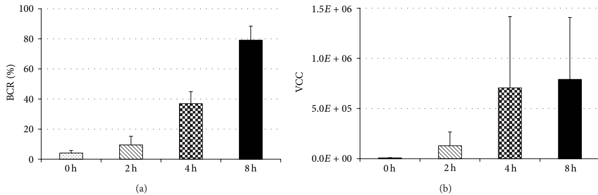
FIGURE 1: BCR and VCC after adhesion. After 5-minute adhesion to the washer surface, the bacteria were cultured and formed biofilm in TSB for 0, 2, 4, and 8 hours. BCRs on the washer surface were 4.1, 9.5, 37.0, and 79.2% in the immediate, 2 hr, 4 hr, and 8 hr groups, respectively, showing a significant increase with prolongation of the culture time in TSB (a). VCCs in biofilm were 7.2 \times 10^3 , 1.3 \times 10^5 , 7.0 \times 10^5 , and 7.9 \times 10^5 CFU, respectively, showing no significant difference among the groups (b). Values represent mean and error bars indicate SD ( n = 80 (a), n = 5 (b)).
