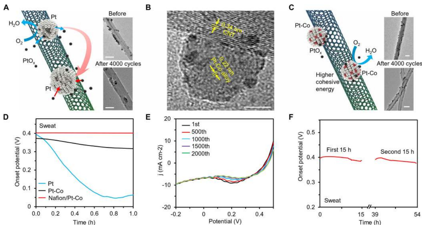
Fig. 3. Characterization of role of Pt alloy nanoparticles in the BFC stability.
