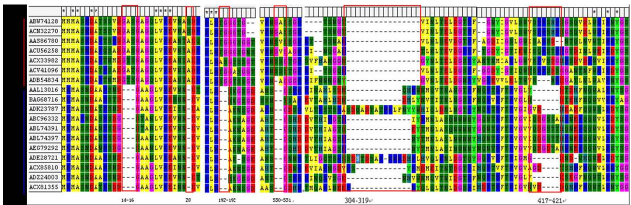
Figure 1 Four sites deletion of GII and unique insertion of GII.3, GII.6 and GII.4. Four sites deletion of GII (14-16)(28)(192-193)(530-531); unique insertion of GII.3 and GII.6 (304-319); unique inserted fragment of GII.4 at 417-421.
