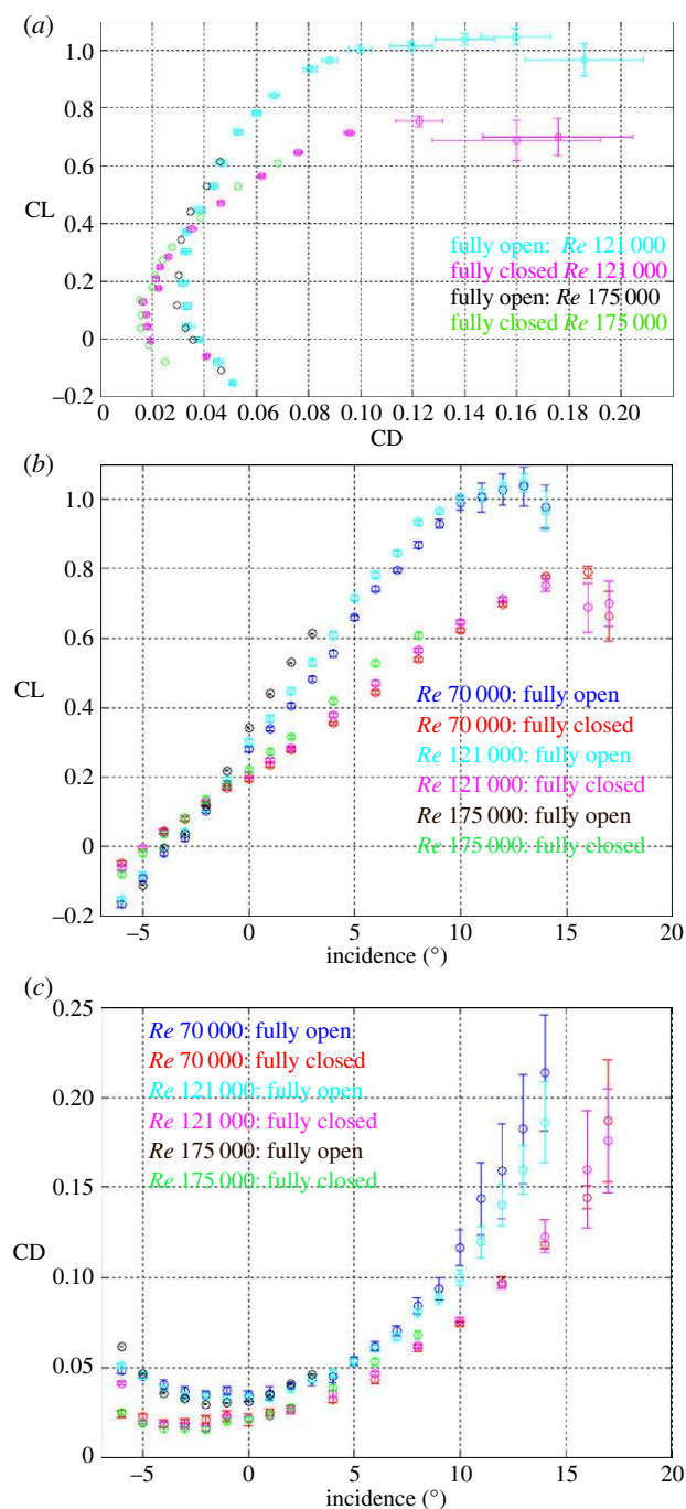
Figure 11. (a) Polar curves of the morphing wing obtained through wind tunnel measurements for Re 121 000 and 175 000 (error bars are fully contained inside the circular markers and therefore not shown). (b) CL and (c) CD as a function of incidence for the three tested values of Reynolds numbers (70 000, 121 000 and 175 000).
