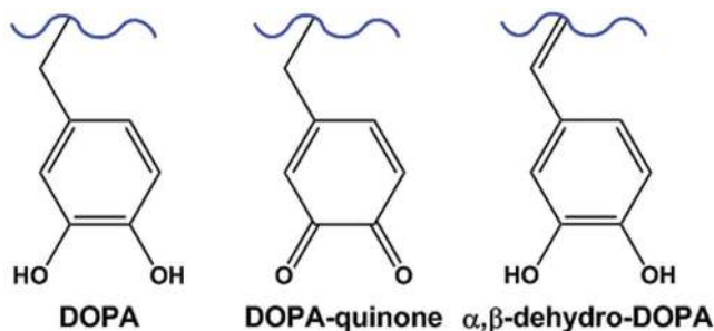
Figure 3. Chemical structures of DOPA, its oxidized form (DOPA-quinone), and the tautomeric form of DOPA-quinone ( \alpha,\beta -dehydro-DOPA).
