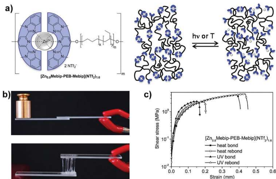
Figure 22. a) Schematic representation of a Mebip-functionalized poly(ethylene-co-butylene) metallo-supramolecular adhesive. Heat or UV light shifts the equilibrium toward the noncoordinated state, leading to softening of the material and thus severely weaker adhesion. b) Images of quartz-glass lap joints before and after fracture. c) As demonstrated by lap-joint experiments, full recovery of the adhesive properties was obtained through a heat or UV treatment. In contrast to a similar UPy-based adhesive, strong UV absorption of the Mebip groups did not require incorporation of a UV sensitizer. Reproduced with permission. [183] Copyright 2014, American Chemical Society.
