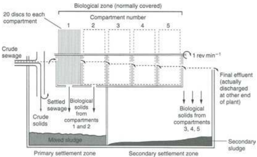
Figure 35. RBC system [1].
