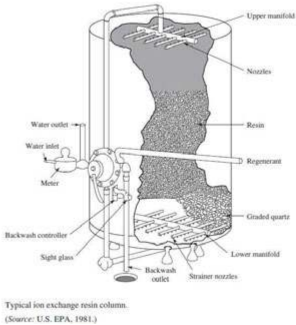
Figure 54. Typical ion exchange resin column [37].
