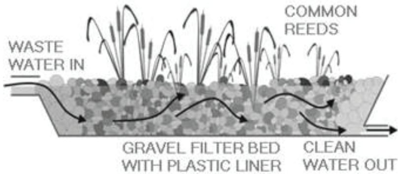
Figure 39. Cross-sectional view of a typical subsurface flow constructed wetland [17].
