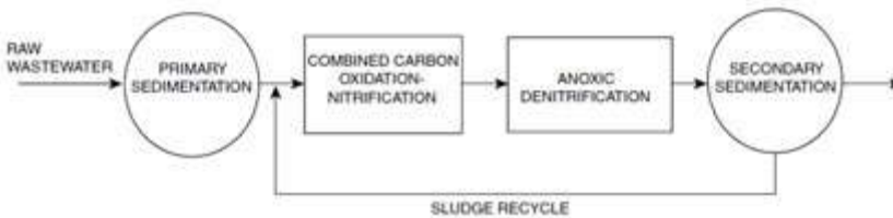
Figure 38. Nitrification/denitrification system for biological removal of nitrogen [3].
