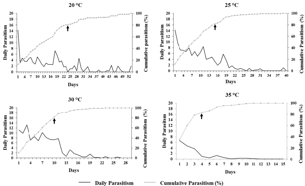
Figure 1. Daily parasitism and accumulation (%) of Telenomus podisi in Euschistus heros eggs at different temperatures [relative humidity of 80±10%, and a photoperiod of 14/10 h (light/dark)]. The arrows indicate 80% parasitism
