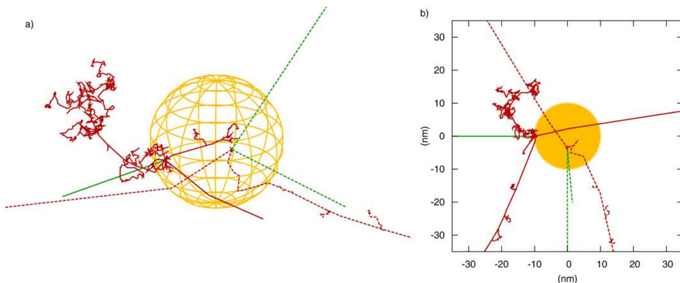
Figure 2 | Comparison of track structure of ionising events either on the surface (solid lines) or in the bulk (dashed lines) of a 20 nm spherical gold nanoparticle, plotted both in 3D (plot a), and as a 2D projection (plot b). Here, an incident 50 keV photon (green tracks) interacts with the gold nanoparticle and ejects a number of electrons (red tracks). For the event which occurs in the bulk, the majority of low-energy electrons are stopped immediately in the nanoparticle, allowing only the most energetic and sparsely ionising electrons to escape. By contrast, the surface event also produces a very large shower of low energy electrons who deposit their energy very densely in the vicinity of the nanoparticle, leading to high doses and many ionising events in a small volume.
