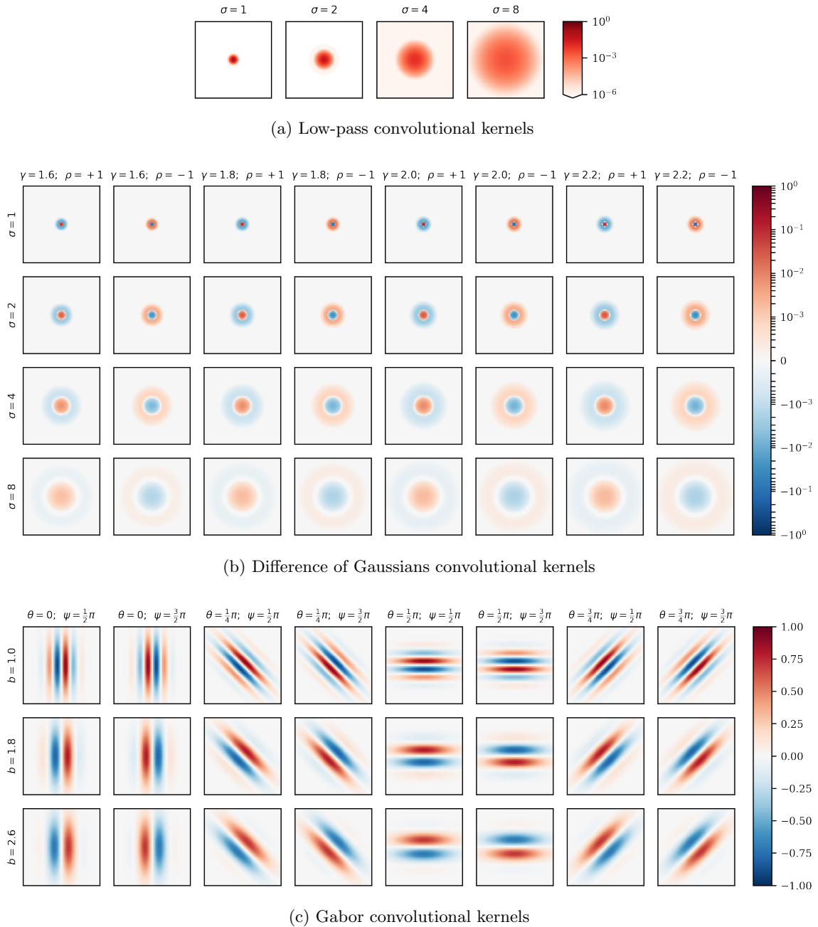
Figure 1: Illustration of the banks of fixed kernels used in the first convolutional layer(s).
