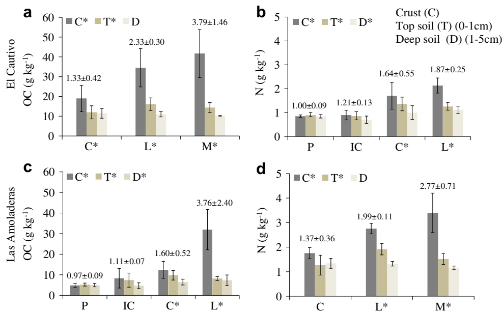
Fig. 1. Mean ( \pm SD, n = 4 ) organic carbon content (OC) (a) and total nitrogen (N) (b) at El Cautivo, and OC (c) and N (d) at Las Amoladeras, in the three soil layers per crust type. Numbers correspond to the crust-underlying soil (including the top and deep soil layers) ratio for each crust type. The crust types are: P, physical crust; IC, incipient-cyanobacterial BSC; C, cyanobacteria-dominated BSC; L, lichen-dominated BSC; M, moss-dominated BSC. *Significant planned contrast. An asterisk (*) next to the name of the soil layer indicates a significant increase in the variable with crust development in that layer. The same symbol next to the name of the crust type indicates a significant decrease in the variable with depth (from the crust towards the 5-cm-deep soil layer) in the specified crust type.
