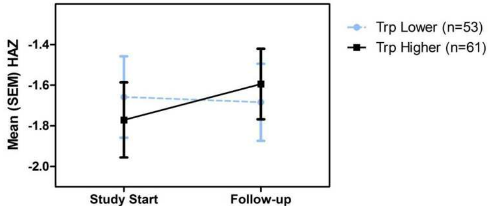
Fig 3. Plasma citrulline (in girls) and tryptophan (in boys) predicts subsequent better growth. A. citrulline (for which gender differs significantly) in girls ( p < 0.001 ; n = 131 ; median citrulline = 23.97 \mu\text{mol/L} ) and B. tryptophan in boys ( p = 0.010 ; n = 114 ; median tryptophan = 66 \mu\text{mol/L} ) predicts subsequent better growth.
