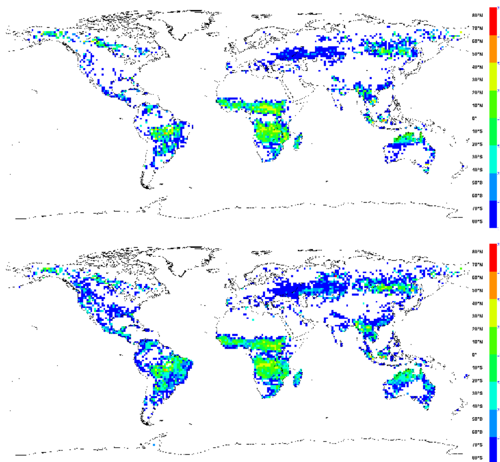
Fig. 5. Average distribution of carbon combustion [ \text{g(C) a}^{-1} \text{m}^{-2} ] during 2003–2008 in GFED3.1 (top) and GFASv1.0 (bottom). Equidistant cylindrical projection, 0.5^\circ resolution. (ECMWF experiment IDs fhhi and ffxr)
