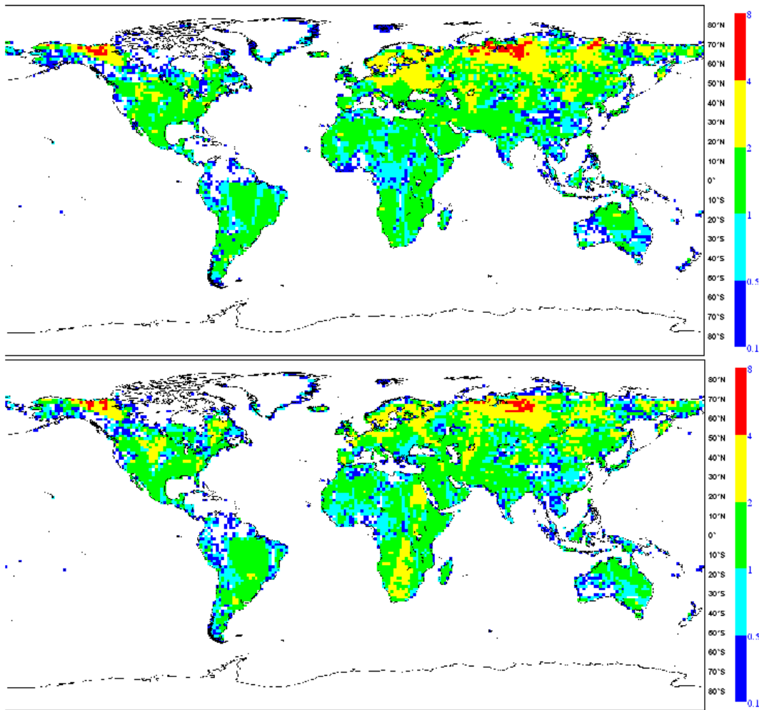
Fig. 2. Effective number of satellite observations of grid cells ( \eta_j \gamma_j ) by MODIS on Terra (top) and Aqua (bottom) on 4 June 2011, 00:00–24:00 UTC. Equidistant cylindrical projection, 0.5^\circ resolution. (ECMWF experiment IDs fbl5 and fbl7)
