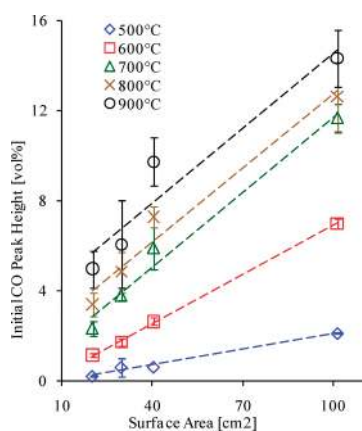
Figure 3. Initial peak height of the gas pulse as a function of the total surface area of particles in the reactor.
