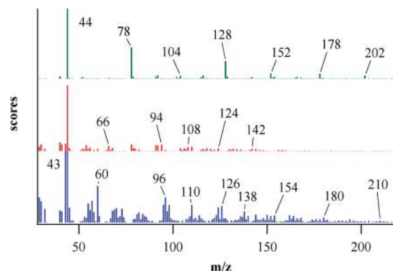
Figure 12. Component scores obtained from MCR analysis of the MBMS data of the pyrolysis of oak spheres in the 4FBR. From top to bottom, PC3 is green, PC2 is red, and PC1 is blue. The scores correspond to the relative molar concentration of each m/z ratio.
