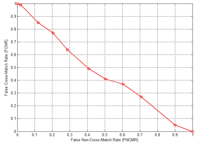
FIGURE 7: FCMR versus FNCMR tested on FVC2002 DB2 when Y = 300 .
