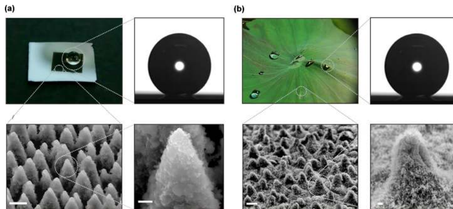
FIG. 5. (a) Top left: picture of a water droplet on an artificial structured silicon surface (dark area). Top right: static contact angle measurement of a water droplet of 0.78 mm radius on that surface; the contact angle is 154^\circ \pm 1^\circ . Bottom left: SEM image of the artificial surface comprising protrusions with conical or pyramidal asperities (scale bar 5 \mu\text{m} ). Bottom right: high magnification SEM image of a single protrusion depicting nanostructures of sizes up to few hundred nanometers on the slopes of the protrusions (scale bar 1 \mu\text{m} ). The surface was structured in the presence of 500 Torr \text{SF}_6 at a laser fluence of 2.47 \text{ J}/\text{cm}^2 with an average of 500 pulses. (b) Top left: picture of water droplets on a Nelumbo nucifera (lotus) leaf. Top right: static contact angle measurement of a water droplet of 0.78 mm radius on the lotus leaf surface; the contact angle is 153^\circ \pm 1^\circ . Bottom left: SEM image of the leaf surface (scale bar 5 \mu\text{m} ). Bottom right: high magnification SEM image of a single papillose depicting branch like protrusions with a size of about 150 nm (scale bar 1 \mu\text{m} ). Reproduced with permission from V. Zorba et al. , Adv. Mater. (Weinheim, Ger.) 20, 4049 (2008). Copyright 2008. Wiley-VCH Verlag GmbH & Co. KGaA.
