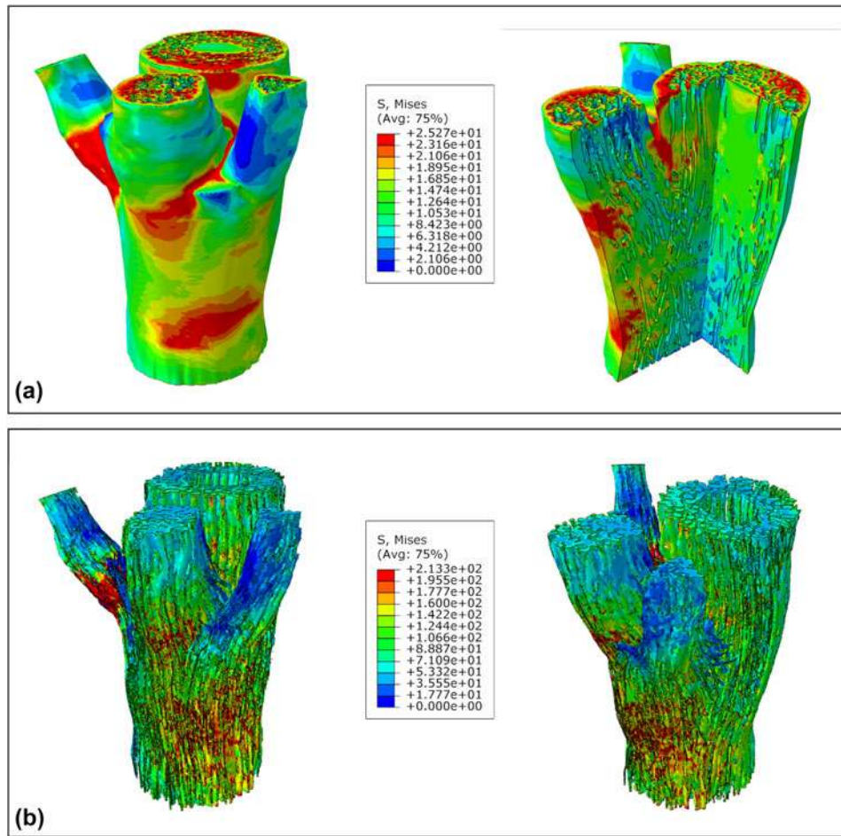
Figure 6: The von Mises stress results at the compressive failure of the \mu CT-based FEA of the nodal region of bamboo: (a) parenchyma elements set only, and internal view cut; (b) sclerenchyma elements set only. Mesh elements contours were hidden to improve the visualization of the colored regions.
