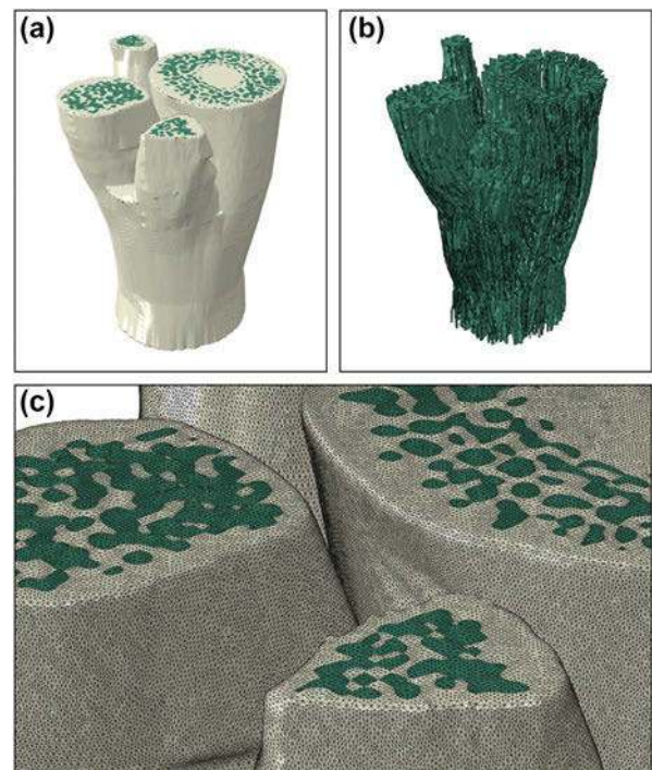
Figure 5: Meshing process for the FEA of the \mu CT-based nodal region of bamboo: (a) discretized assembly model with the regions of parenchyma (white) and sclerenchyma (green); (b) sclerenchyma region only, by hiding the parenchyma mesh elements; (c) detail of the tetrahedral mesh of the assembly. Mesh elements contours were hidden in A and B to improve the visualization of the 3D model.
