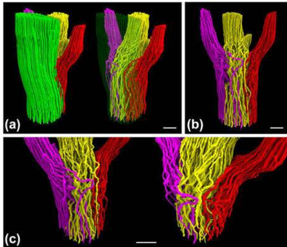
Figure 3: 3D reconstruction of vascular bundles from \mu CT of the nodal bamboo region with secondary branching: (a) vascular bundles of the main axis interweaving with the ones of the secondary axes; (b) vascular bundles of the secondary axes only; (c) details of the transversal movement of secondary vascular bundles. Scale bars = 1 mm.
