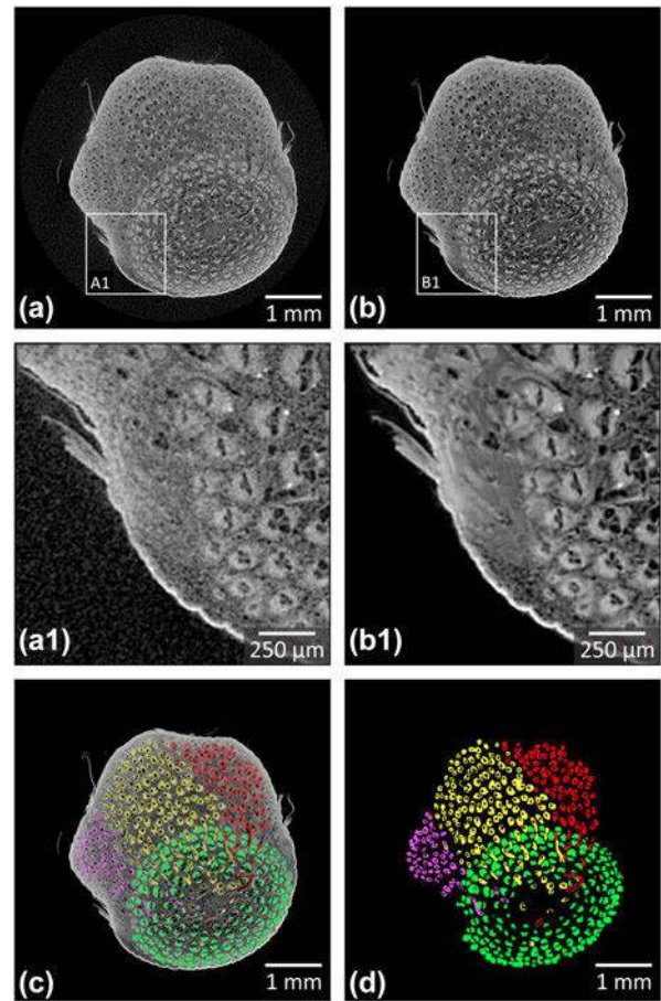
Figure 8: X-ray microtomography image stack processing on nodal bamboo sample: (a) original slice and detail (a1) of the noise in a region; (b) image filtered with non-local means denoising filter and detail (b1) of the same region after noise reduction; (c) manually segmented sclerenchyma of vascular bundles from primary axis (green) and secondary axes (purple, yellow, and red); (d) binary masks of segmented bundles.
