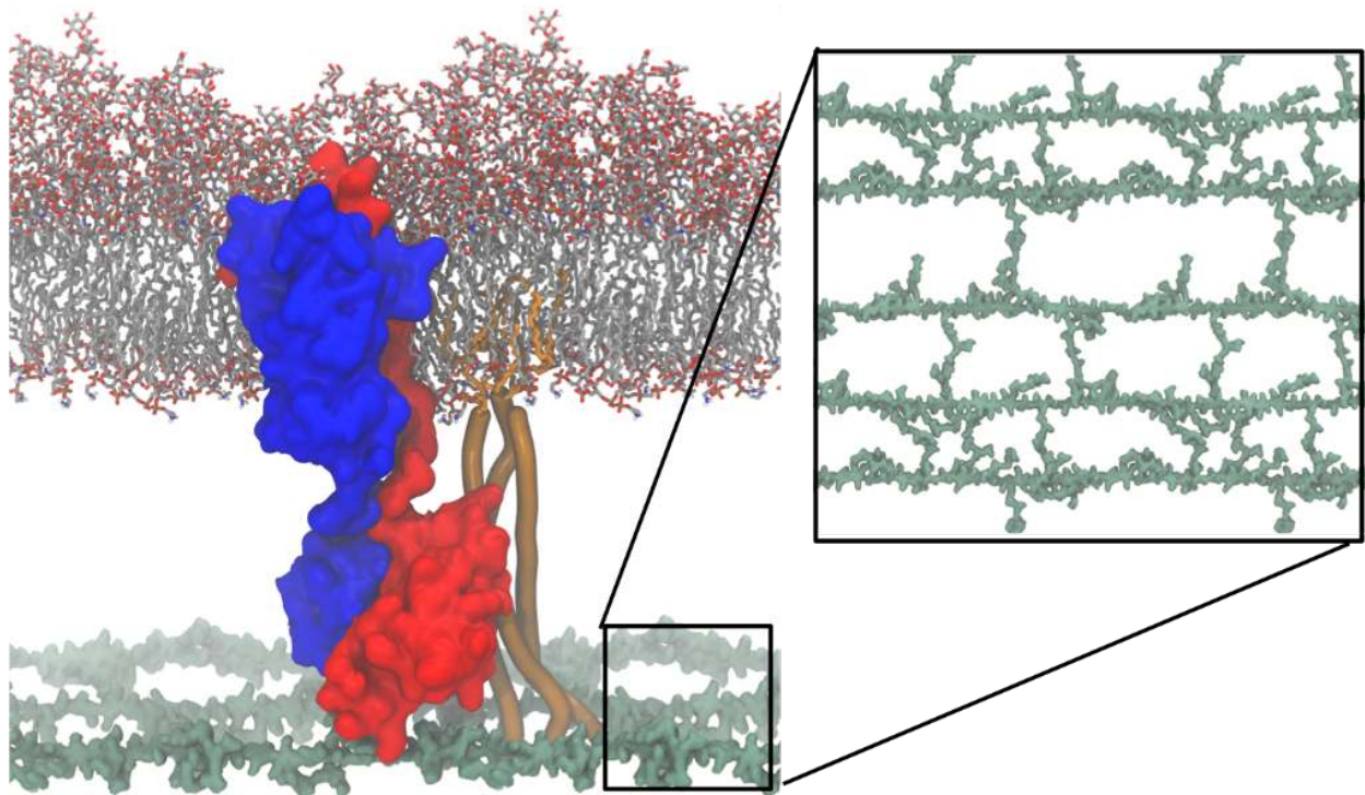
Figure 7 - The outer membrane protein OmpA is shown in its dimeric form in red and blue. Braun's lipoprotein, which is covalently bound to peptidoglycan is shown in orange. Peptidoglycan is shown in green. The lipids of the outer membrane of E. coli are shown in grey and red.(Samsudin, Boags, Piggot, & Khalid, 2017)
