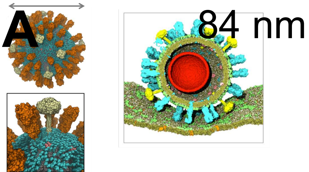
Figure 8 - The viral envelope membrane of influenza A modelled at coarse-grained resolution. The hemagglutinin, neuraminidase, and M2 proteins are orange, yellow and pink respectively. The glycolipid molecules are shown in cyan, and other lipids in grey. Overall (A) and zoomed-in (B) views are shown. C Model of an influenza A virion (with the red sphere indicating the approximate location of the genome within the virion, not currently modelled) docked against a simple model of a mammalian cell membrane(Koldsø & Sansom, 2015) with glycolipids in pale green, other lipids in darker green, and cell membrane proteins in orange.
