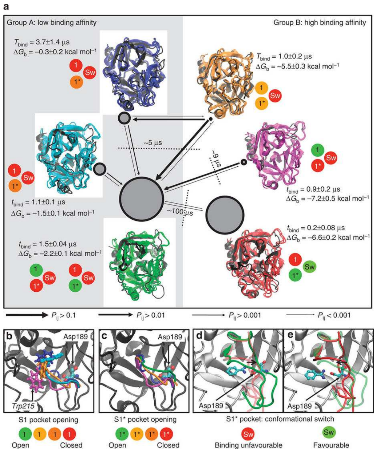
Figure 1 - Example of a typical Markov-state model (MSM). In this case, the MSM describes structural features, equilibrium distribution, and kinetics of six unbound (apo) trypsin conformations (a). Transitions between them occur at timescales on order of tens of microseconds. The three slowest relaxation timescales and their corresponding transition process are indicated (dashed lines). The circles have an area proportional to the equilibrium probability \pi_i . The respective free energy differences \Delta G_b of binding a ligand to these six conformations and the binding time t_{\text{bind}} (mean first passage time to binding) are given. The arrows indicate the transition probabilities for direct transitions between the different states (see legend). The most important structural differences concerning ligand binding are shown in b–e, and the structures are classified with respect to these
