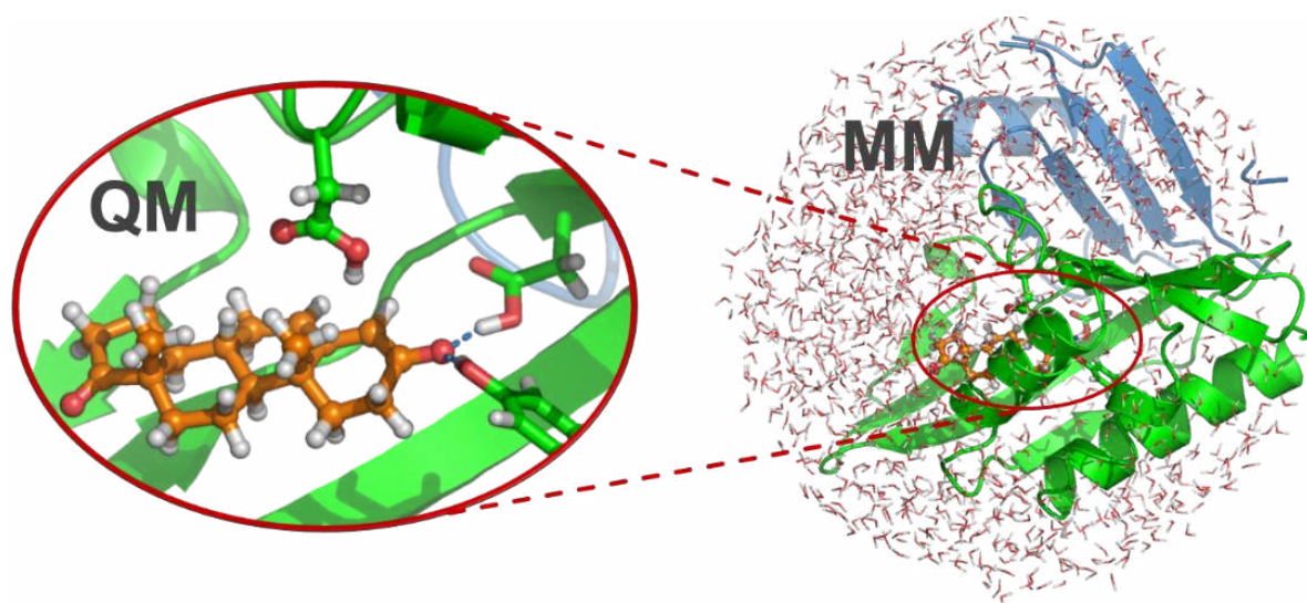
Figure 3 - Example of QM/MM modelling of an enzyme-catalysed reaction. The enzyme (ketosteroid isomerase) is divided into an MM region and a QM region. The intermediate structure after the first proton transfer in the mechanism is shown.(van der Kamp, Chaudret, & Mulholland, 2013)
