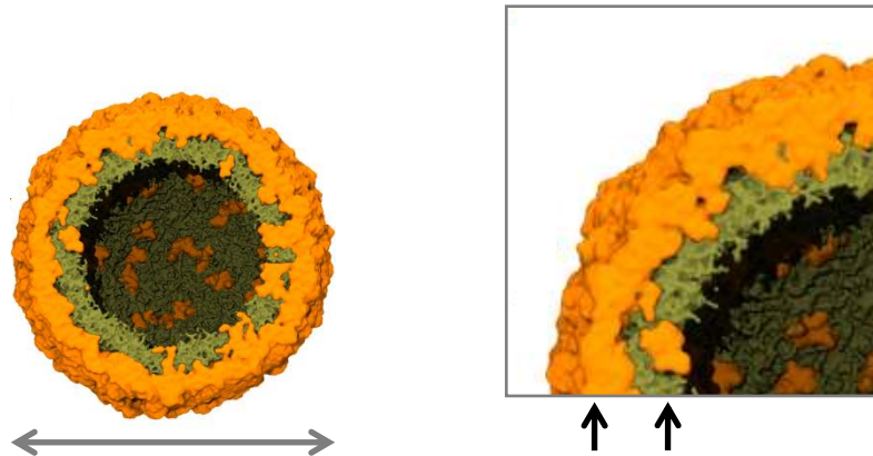
Figure 9 - A coarse-grained model of the envelope of dengue virus (Reddy & Sansom, 2016b) shown as (A) a cross-section of the entire virion envelope model is shown, along with (B) a zoomed-in view. Protein (orange) and lipid (dark green) components of the envelope are shown.
