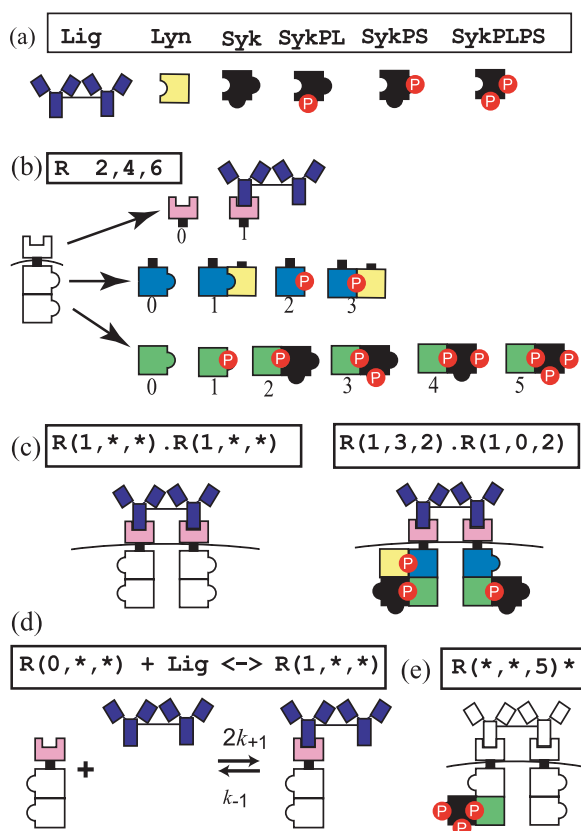
Fig. 1. Illustrated declarations in the input file ( fceri_net.in ) that specifies the model and output functions of Faeder et al. (2003). Boxes enclose text of the input file. (a) Declarations of six individual molecular species. (b) A multistate species declaration of 48 individual molecular species that contain one receptor (R). Each of these species is characterized by three domains, which have two, four and six possible states. (c) Declaration of complexes that contain two receptors (left) and a reference to one of the 300 individual molecular species in this class (right). (d) The reaction rule for ligand–receptor binding, which implies 24 distinct forward reactions and the same number of reverse reactions. All forward (reverse) reactions are assigned the rate constant k_{+1} ( k_{-1} ). (e) Declaration of an output function, a weighted sum of 98 concentrations, used to calculate the total concentration of autophosphorylated Syk.
