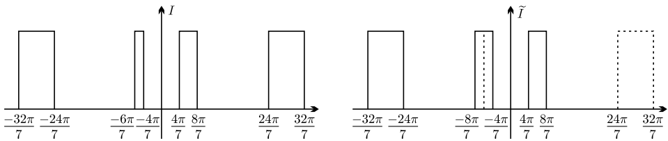
Fig. 5.1. The functions |\widehat{\psi}| = \chi_I and |\widehat{\tilde{\psi}}| = \chi_{\tilde{I}} when \alpha = 0 and b \equiv 1
