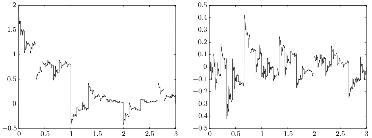
Fig. 4. The functions \operatorname{Re} \tilde{\Phi} (left) and \operatorname{Im} \tilde{\Phi} (right) from Example 3.
