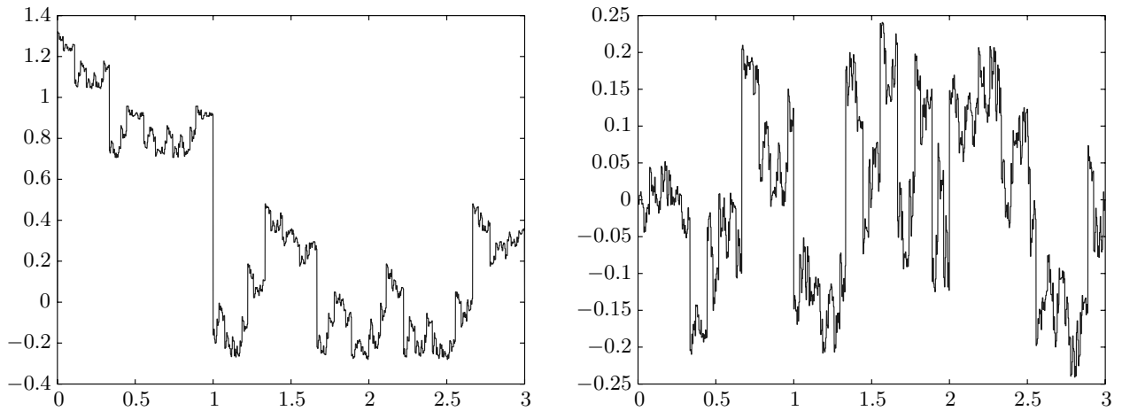
Fig. 3. The functions \operatorname{Re} \Phi (left) and \operatorname{Im} \Phi (right) from Example 3.
