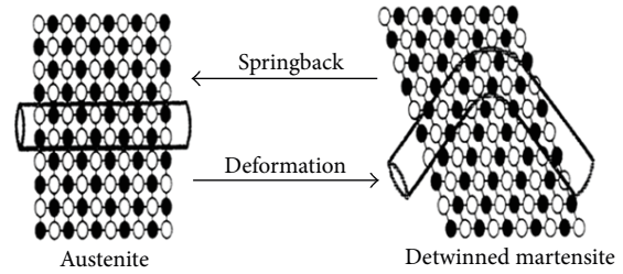
FIGURE 2: Diagrammatic representation of the superelasticity effect of NiTi alloy. Source: [33].
