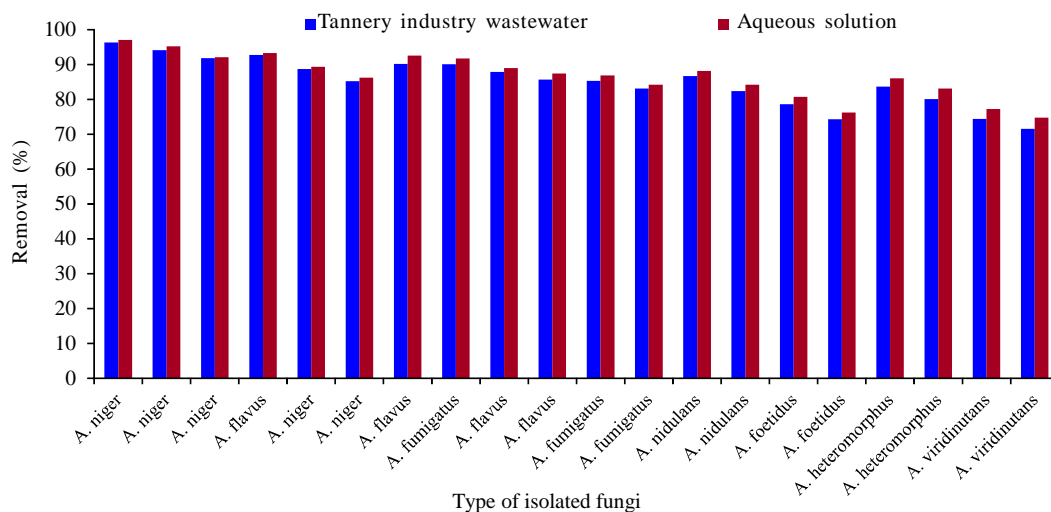
Fig. 4: The maximum removal percentage Cr(VI) in a tannery industry wastewater and in an aqueous solution by an isolated fungi with an optimum pH of 3, optimum incubation time of 7 days, optimum fungus biomass of 4.0 g and an initial Cr(VI) concentration of 18.125 mg/L
