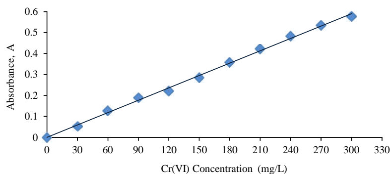
Fig. 3: Calibration curve for standard Cr(VI) ion solution for the maximum absorbance wavelength of 542 nM
