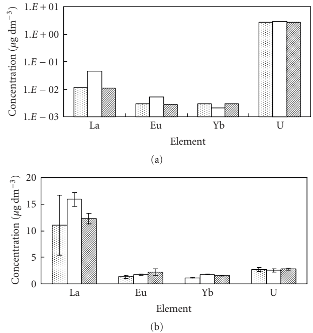
FIGURE 4: The concentrations of REEs and U in seawater samples. (a) Dissolved fraction; (b) suspended solid fraction. (▨): Itoigawa city, (□): Izumozaki town, (▩): Kashiwazaki city.
