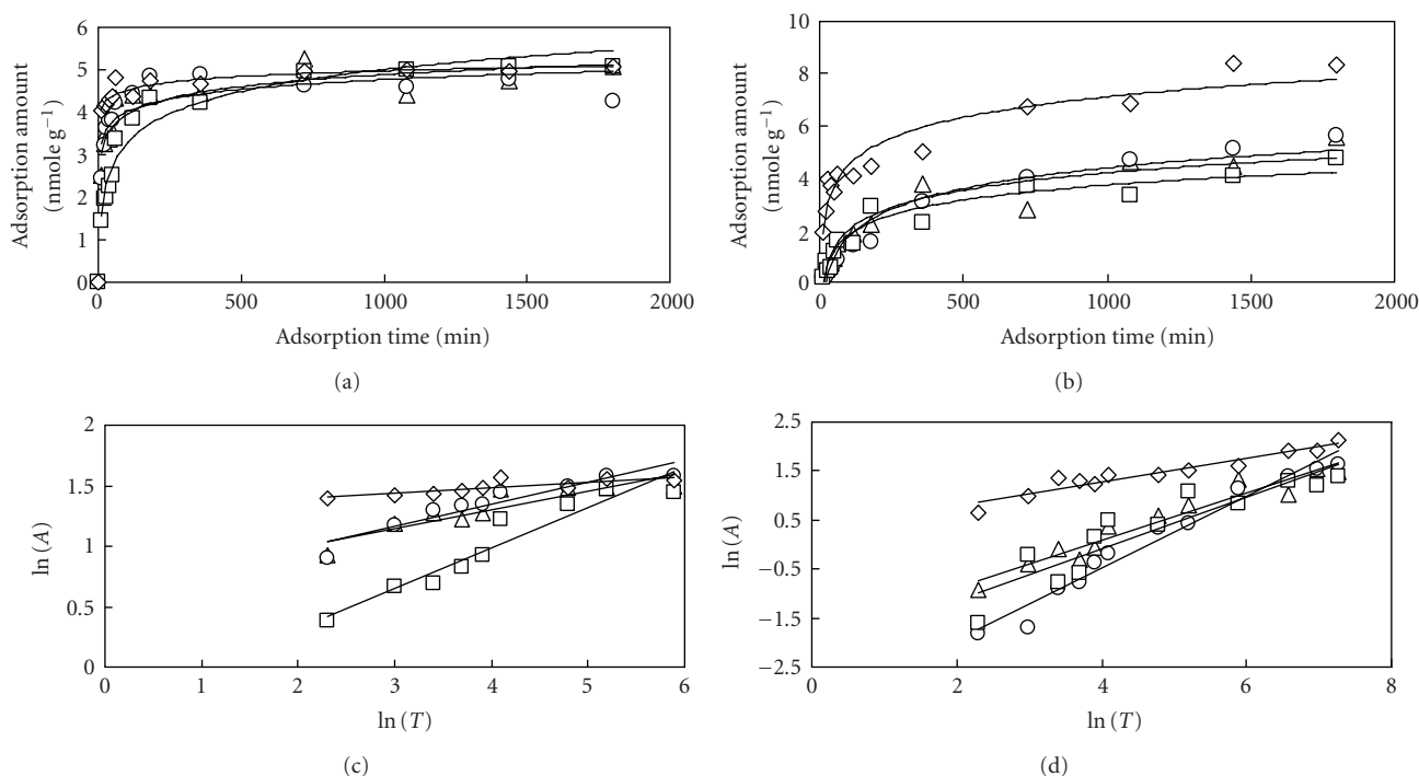
FIGURE 6: The amount of (a) La or (b) U adsorption to each sample. (○): S. h. , (Δ): U. p. , (□): dry U. p. , (◇): alginic acid. The amount of La or U adsorption to each sample. (○): S. h. , (Δ): U. p. , (□): dry U. p. , (◇): alginic acid ((c): La in logarithmical scale, (d): U in logarithmical scale).
