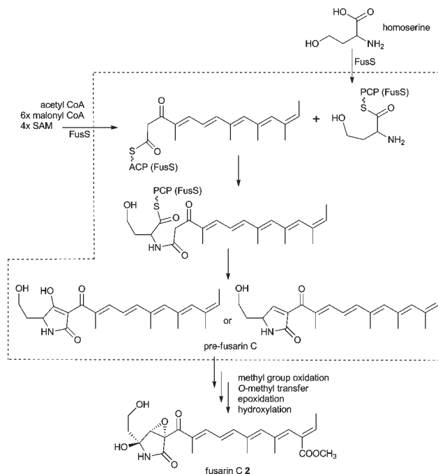
Scheme 1 Proposed fusarin C 2 biosynthesis (structures in the dashed box are proposed compounds).
