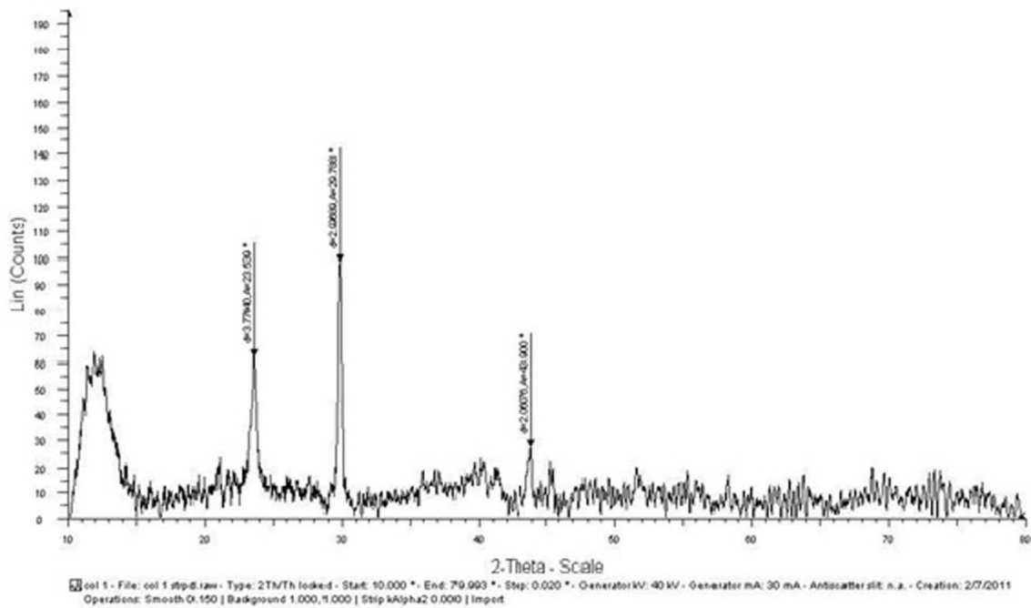
Fig. 6. X-Ray Diffraction Studies of Selenium nanoparticles by Bacillus sp. JAPSK2
