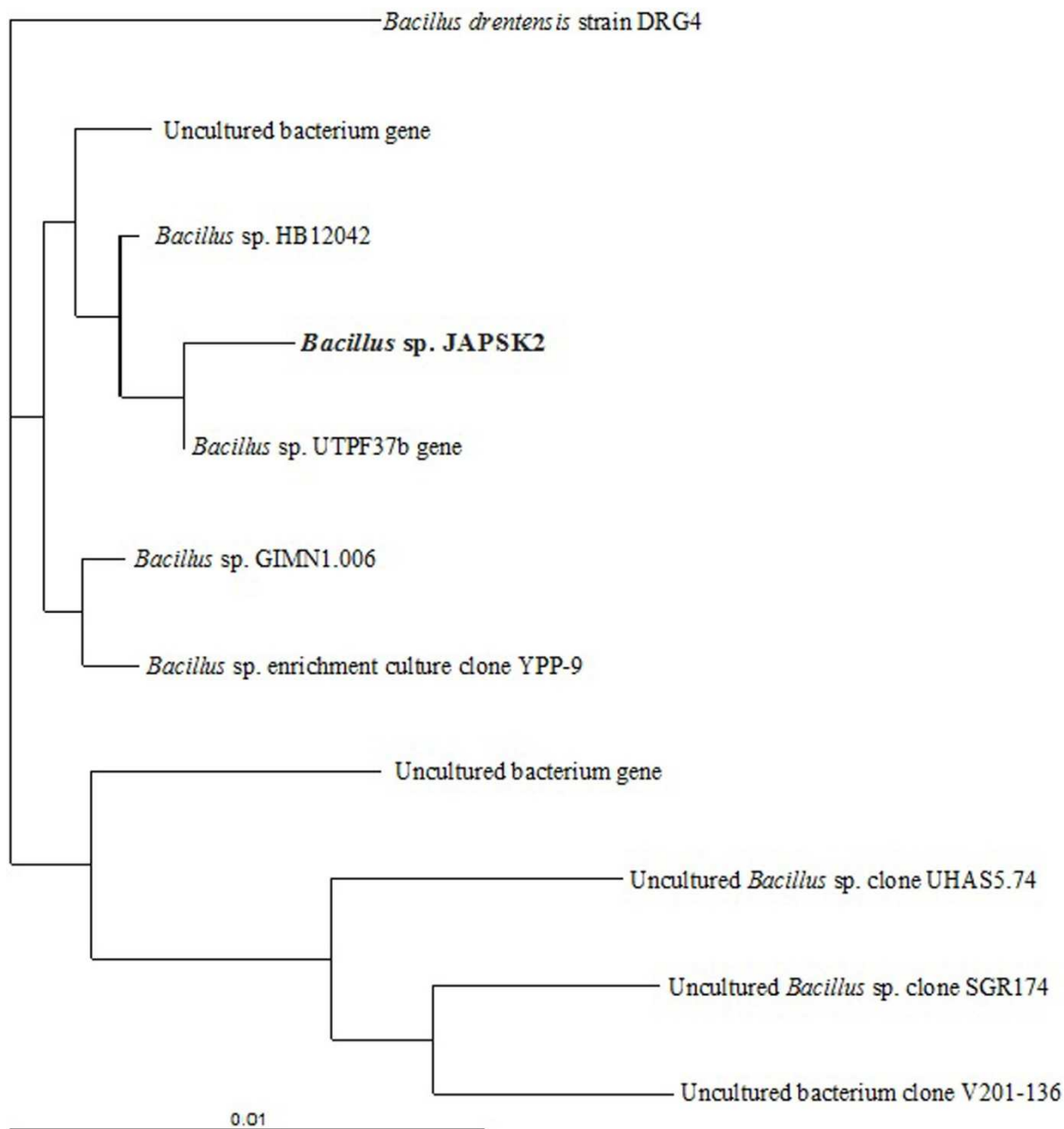
Fig. 1. Phylogenetic tree of Bacillus sp JAPSK2
