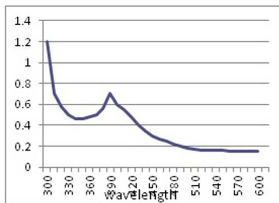
Fig. 2. UV-Vis analysis of Silver nanoparticles synthesised by Bacillus sp. JAPSK2 showing peak at 393nm
