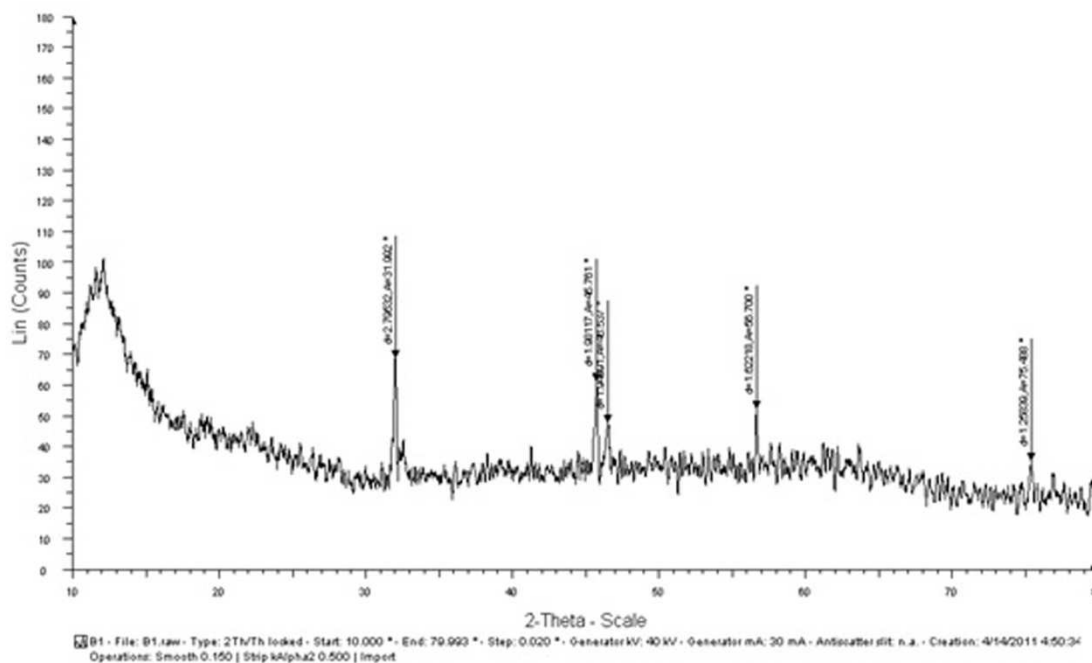
Fig. 3. X-Ray Diffraction Studies of Silver nanoparticles by Bacillus sp. JAPSK2
