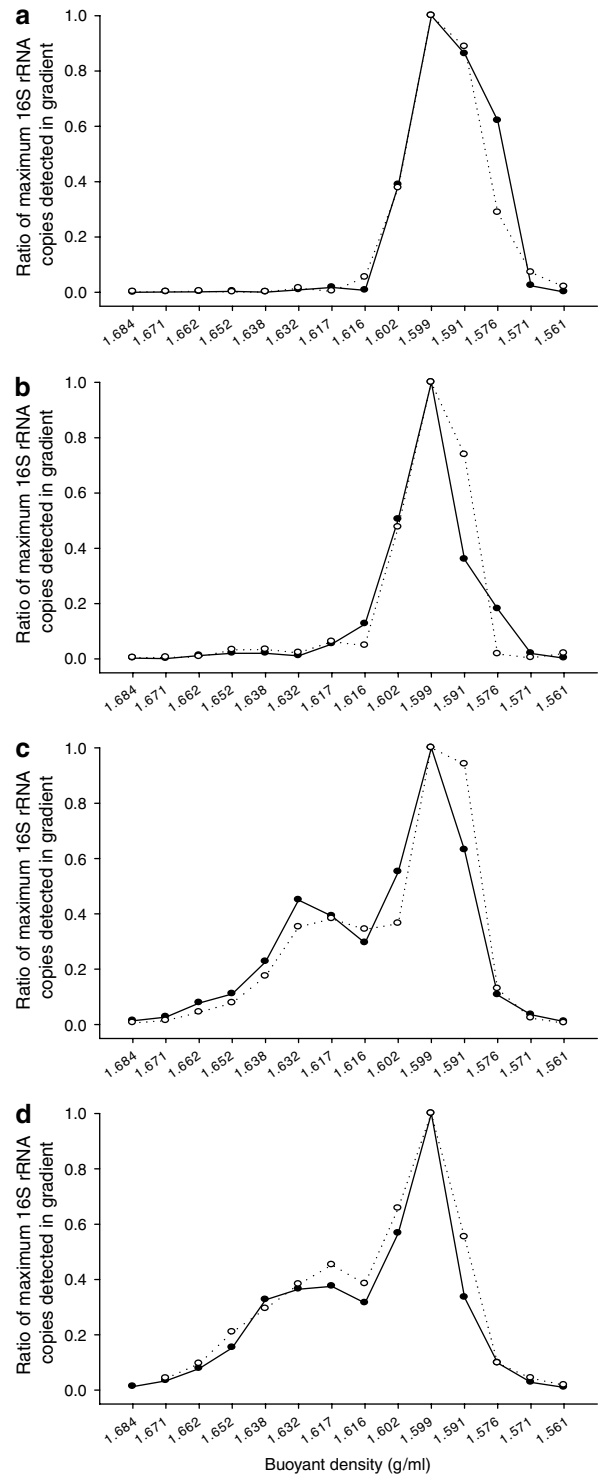
Figure 1 Detection of ^{13}\text{C} -DNA in density gradient fractions derived from DNA at (a) the initiation of the experiment ( t=0 ) and following incubation times of (b) 1 day; (c) 4 days; and (d) 14 days using Q-PCR targeting 16S rRNA genes. (a) (solid symbols) and (b) (open symbols) denote replicate density gradients run for each sample.
