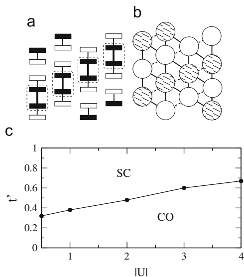
Fig. 3. (a) PEC in the \beta' CTS. Singlets indicated by heavy line and dashed boxes. (b) Effective -|U| , +V , t' , t model. Pairs of singlet-bonded sites (vacancies) are mapped to a single doubly occupied (vacant) site in the effective model. (c) Phase diagram of the effective model for V = 1 [11].
