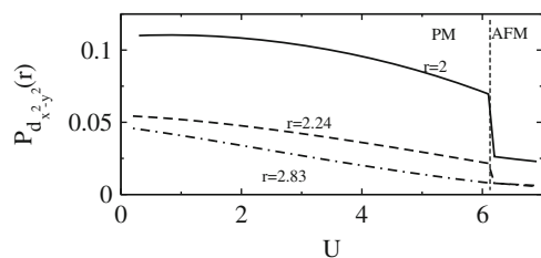
Fig. 1. Exact d-wave SC pair correlation functions versus distance r , for the \frac{1}{2} filled 4 \times 4 periodic anisotropic triangular lattice for t'/t = 0.5 . SC correlations similarly decrease monotonically with increasing U for all t'/t [2].
