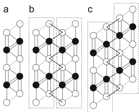
Fig. 2. (a) The \rho = 0.5 zigzag ladder [5]. Ladders combine to form a 2D lattice in two ways, forming either horizontal stripe (b) or diagonal stripe (c) CO patterns. Black and white circles denote charge-rich and charge-poor sites. Double bonds between the charge-rich sites indicate spin singlets.
