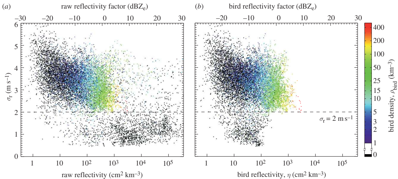
Figure 4. Radial velocity standard deviation \sigma_r as a function of raw reflectivity (a, reflectivity including non-bird echoes) and as a function of bird reflectivity (b, reflectivity cleaned from non-bird echoes). Each scatter point refers to a time–height layer, i.e. a specific height layer measured at a specific time. To limit the number of scatter points, only data for the Wideumont campaign are shown (22 September–21 October 2007, 14 742 detected non-empty time–height layers). In colour, the bird density is indicated as measured simultaneously by the bird radar. The large majority of non-zero bird densities are observed for time–height layers with \sigma_r > 2 \text{ m s}^{-1} .
