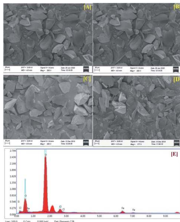
Fig. 2 Characterisation of the SiO 2 -FeCl 3 catalyst: [A] SEM images of 230–400 mesh, [B] SEM images of freshly prepared SiO 2 -FeCl 3 , [C] six-month-old SiO 2 -FeCl 3 , [D] recycled SiO 2 -FeCl 3 and [E] EDAX spectrum of SiO 2 -FeCl 3 showing absorption peaks for Fe, Cl, Si and O.
