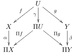
Fig. 1. Bisimulation as a span in a coalgebra category.
