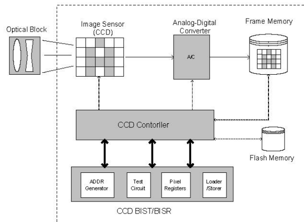
Fig. 1. BIST/BISR Architecture
