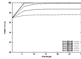
Fig. 12. Test and Repair (3 Test Circuit and Hard Yield=97%)
