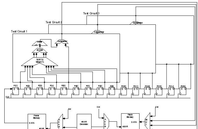
Fig. 5. The proposed BIST circuit (3 Test Circuit)
