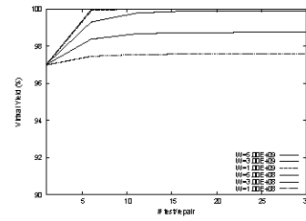
Fig. 15. Test and Repair (5 Test Circuit and Hard Yield=97%)
