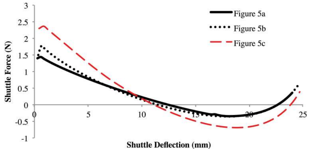
Fig 6. Comparing geometry of compliant segments. The thicker segments increase the force slightly.
