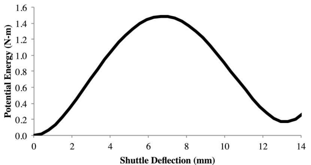
Fig 8. Predicted energy curve of the metallic glass bistable mechanism from the PRBM.
