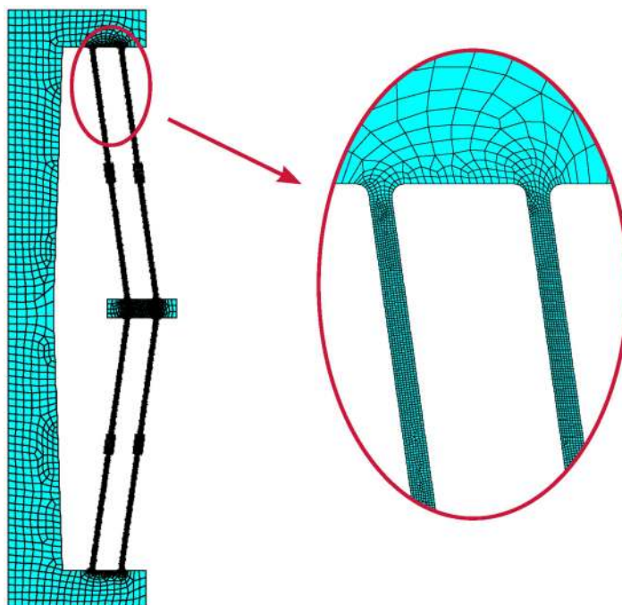
Fig 10. An example of the finite element mesh for the bistable mechanism.
