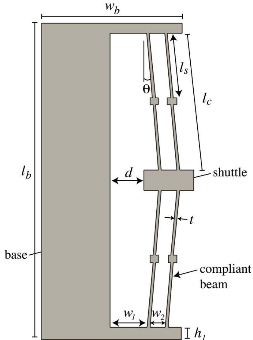
Fig 2. Labeled bistable mechanism.
