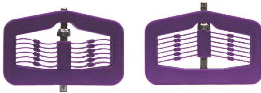
Fig 14. Prototype of a pin-puller non-explosive release mechanism in its second stable position (left) and its fabricated position (right).
