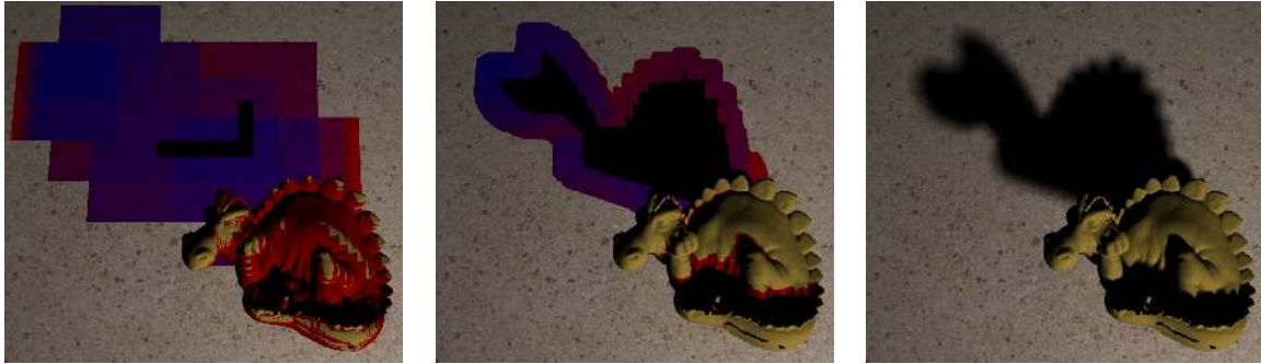
Figure 8: HSM (left) vs. MSSM (center): pixels for which some micropatches have to be backprojected to determine the actual degree of the light's occlusion are highlighted (red: at most 6 \times 6 patches at an effective shadow map resolution of 256^2 need to be processed, blue: at least 20 \times 20 patches). Right: resulting soft shadow.
