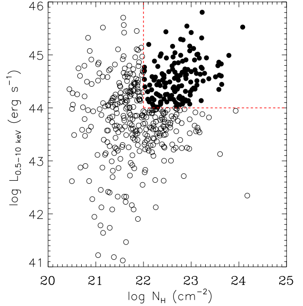
Fig. 1. X-ray luminosity in the [0.5–10 keV] band corrected for obscuration plotted against the N_H column density for the X-ray sources in the XMM-COSMOS survey with a redshift. The 142 Type-2 QSOs studied in this paper are indicated by filled circles. The dashed lines delimit the area where L_{[0.5-10 \text{ keV}]} > 10^{44} \text{ erg s}^{-1} and N_H > 10^{22} \text{ cm}^{-2} .
