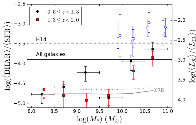
Figure 11. Same format as Figure 8, but for star-forming galaxies. The solid horizontal line indicates the best-fit intercept in Figure 4.
