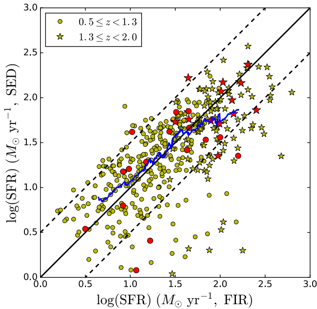
Figure 3. Comparison between SFRs derived from SED fitting and those derived from FIR photometry. Circles and stars indicate sources in the redshift ranges of 0.5 \leq z < 1.3 and 1.3 \leq z < 2.0 , respectively. Their FIR-based SFRs are derived from 100 and 160 \mu\text{m} observations with Herschel /PACS, respectively (see Section 2.2). Red symbols indicate AGNs selected by their large X-ray luminosities ( L_X > 3 \times 10^{42} \text{ erg s}^{-1} ; see, e.g., L17). The black solid line indicates a 1:1 relation between two SFR measurements; the dashed lines indicate 0.5 dex offsets. Our adopted SFRs (from SED fitting) generally agree with those derived from FIR photometry. The blue solid curve indicates running median SFR offsets from bins of 50 sources. For X-ray-luminous AGNs, the SED-based SFRs do not have significant systematic differences relative to FIR-based SFRs.
