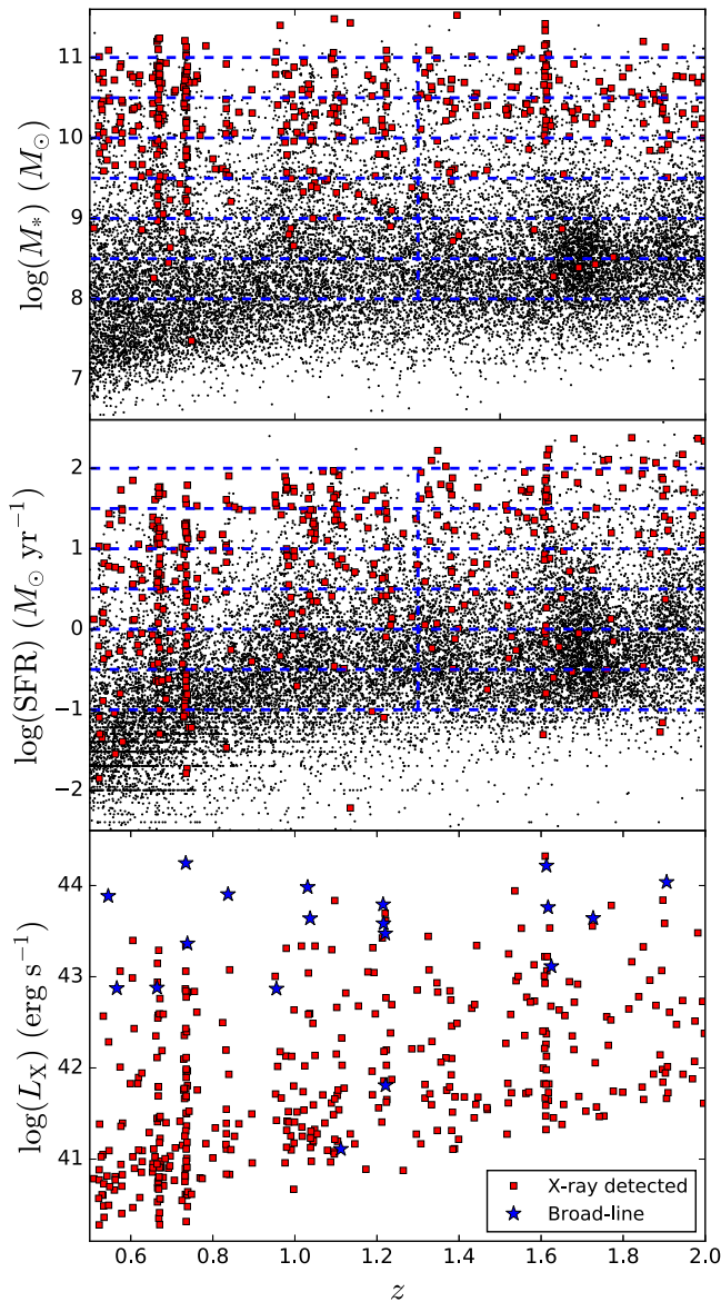
Figure 1. M_* (top) and SFR (middle) vs. redshift for all our sources. The red squares indicate X-ray detected sources. The blue dashed lines indicate our binning grids in Figures 4, 5, and 8. The bottom panel presents absorption-corrected L_X (see Section 2.3) as a function of redshift for X-ray detected sources. The blue stars indicate broad-line AGNs that are excluded from our sample. The overdensities at z \approx 0.7 and 1.6 are likely due to cosmic variance (e.g., Silverman et al. 2010; Finoguenov et al. 2015; L17).
