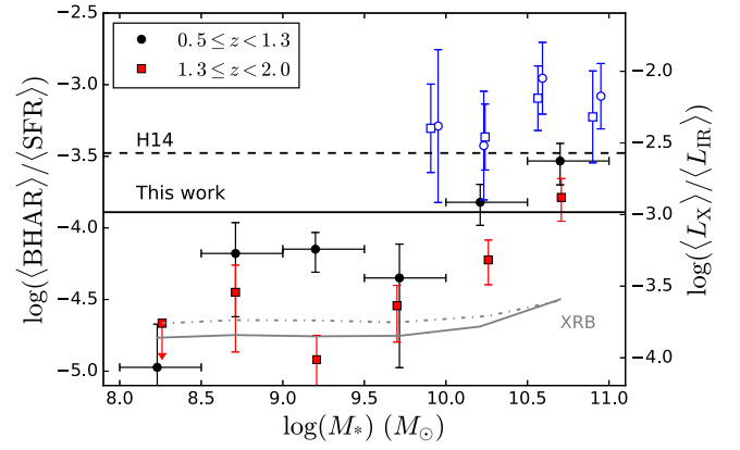
Figure 8. Ratio of \langle \text{BHAR} \rangle to \langle \text{SFR} \rangle as a function of M_* . The black points and red squares indicate sources in the low- z and high- z ranges, respectively. Their horizontal positions indicate median M_* in the bin, and the horizontal error bars (only shown for the low- z bin) indicate the bin width. The blue open symbols indicate results from Mullaney et al. (2012a); the circles and squares indicate their z \sim 1 and z \sim 2 samples, respectively. The scale of \langle L_X \rangle / \langle L_{\text{IR}} \rangle is shown on the right side, where we convert SFR to L_{\text{IR}} with a constant factor (C13). The gray solid and dotted-dashed lines indicate the \langle L_X, \text{XRB} \rangle / \langle L_{\text{IR}} \rangle ratios in the low- z and high- z ranges, respectively. These values are used as upper limits for \langle L_X \rangle / \langle L_{\text{IR}} \rangle for AGNs, when 1\sigma lower limits of \langle L_X \rangle for AGNs are negative. The solid horizontal line indicates the intercept of our best-fit \langle \text{BHAR} \rangle -SFR linear relation in Figure 4; the dashed horizontal line indicates the H14 model. The \langle \text{BHAR} \rangle / \langle \text{SFR} \rangle ratio is strongly dependent on M_* . More massive galaxies generally have higher \langle \text{BHAR} \rangle / \langle \text{SFR} \rangle , indicating that they are more efficient in growing their SMBHs. For high-mass galaxies ( M_* \gtrsim 10^{10} M_\odot ), our \langle \text{BHAR} \rangle / \langle \text{SFR} \rangle values are systematically lower than those in Mullaney et al. (2012a). This is likely caused by the exclusion of broad-line AGNs in our sample (see Sections 2.1 and 3.5.1).
