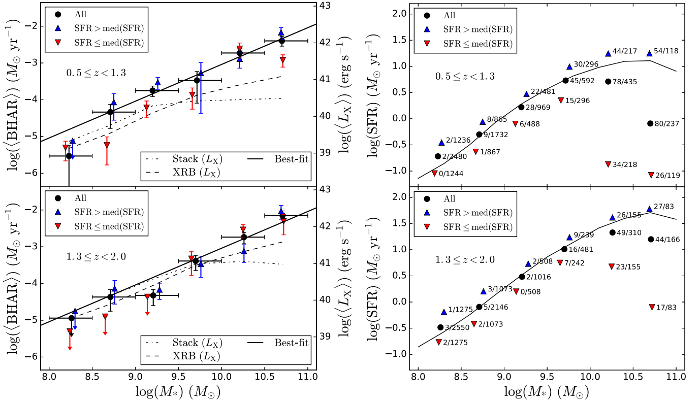
Figure 5. Same format as Figure 4, but the bins are based on different M_* (x-axis), and each sample is split into two subsamples based on SFR. \langle \text{BHAR} \rangle is positively correlated with M_* . The solid curves in the right panels indicate the star-forming main sequence (B13).
