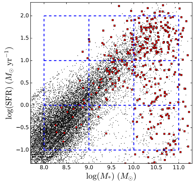
Figure 2. SFR vs. M_* for all our sources. The red squares indicate X-ray detected sources. The blue dashed lines indicate our binning grids in Figure 6.
