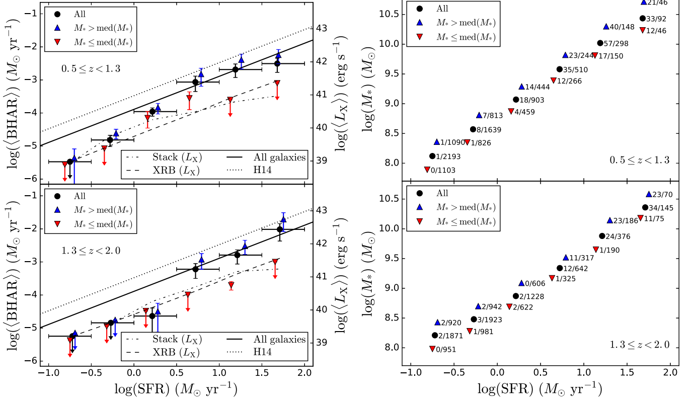
Figure 9. Same format as Figure 4, but for star-forming galaxies. The black solid line indicates the fitting of all galaxies as in Figure 4, rather than the fitting of star-forming galaxies.
