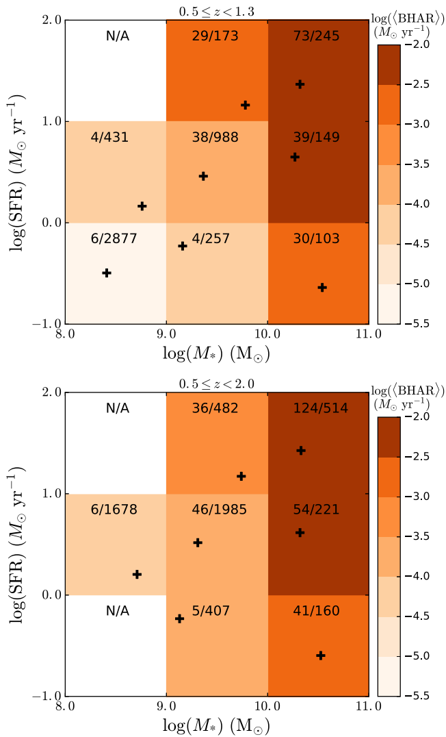
Figure 6. Color-coded \langle \text{BHAR} \rangle as a function of SFR and M_* at 0.5 \leq z < 1.3 (top panel) and 0.5 \leq z < 2.0 (bottom panel). The text in the center of each square indicates the number of X-ray detected sources and all sources. The black plus sign indicates median values of SFR and M_* for sources in each bin, which are adopted in the analyses in Section 3.3. In both panels, the upper left squares with white color include too few sources (fewer than 100; see Section 3.1), and their \langle \text{BHAR} \rangle values are not calculated. In the bottom panel, the \langle \text{BHAR} \rangle of the lower left square has a negative 1\sigma lower limit; its value is not shown. The results for the two redshift bins are similar. Both M_* and SFR have positive correlations with \langle \text{BHAR} \rangle .
