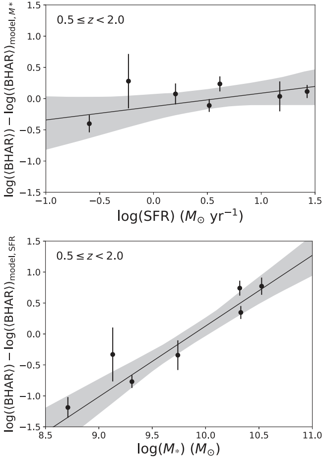
Figure 7. Top: \langle \text{BHAR} \rangle residuals of the \langle \text{BHAR} \rangle - M_* fit as a function of SFR. The black solid line indicates the best fit for the residuals as a function of SFR. The shaded region indicates 3\sigma uncertainties derived from Markov chain Monte Carlo sampling utilizing “emcee” (Foreman-Mackey et al. 2013). The residual-SFR relation is flat. Bottom: \langle \text{BHAR} \rangle residual of the \langle \text{BHAR} \rangle -SFR fit as a function of M_* . The residual- M_* relation is steep.
