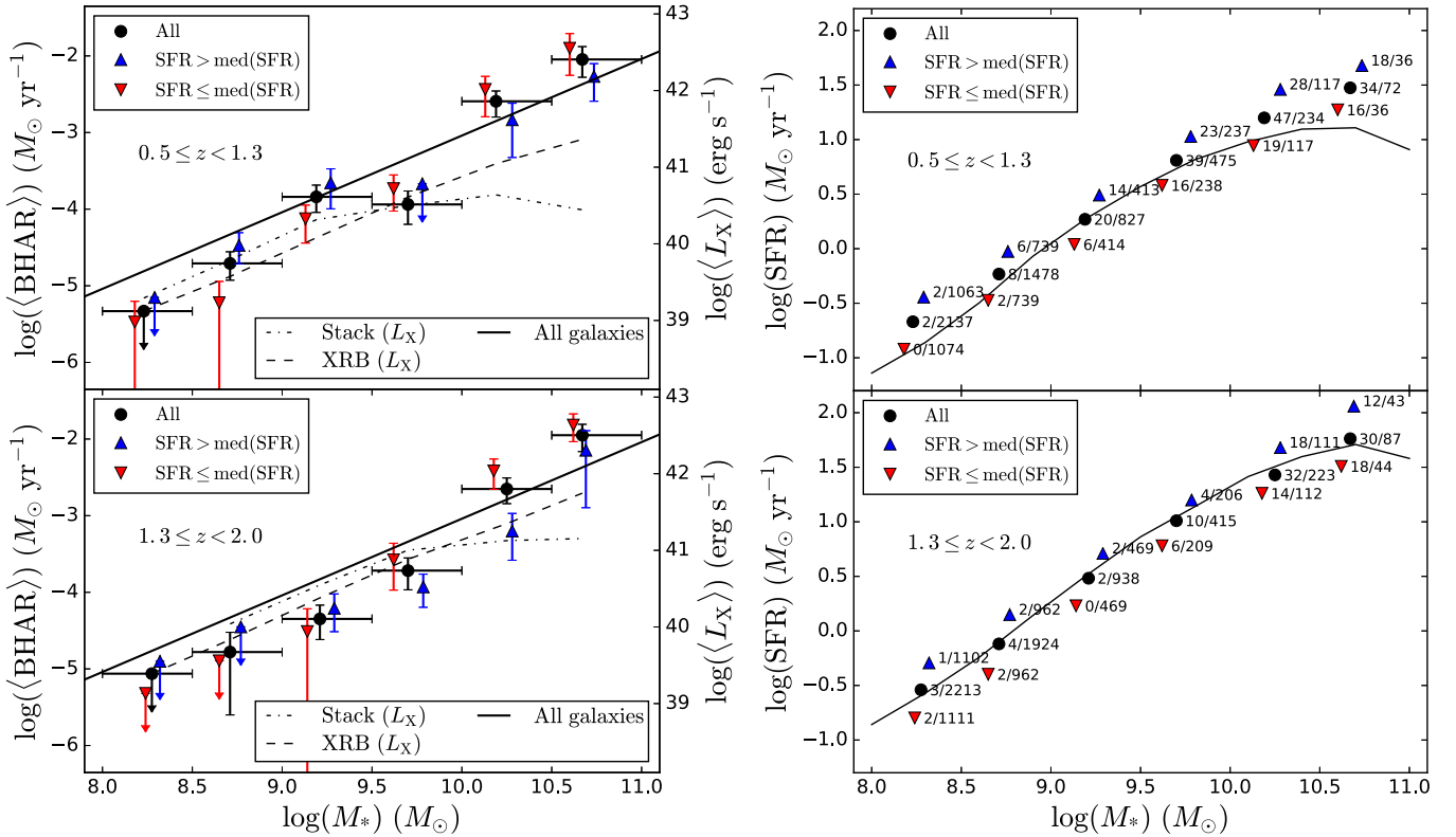
Figure 10. Same format as Figure 5, but for star-forming galaxies. The black solid line indicates the fitting of all galaxies as in Figure 5, rather than the fitting of star-forming galaxies.
