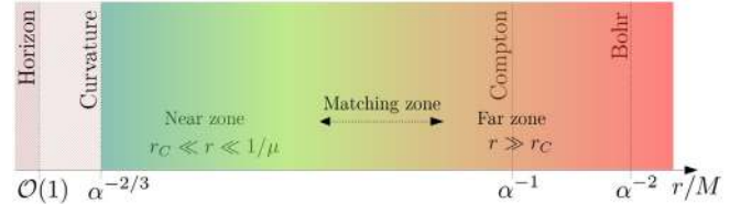
FIG. 1. Schematic representation of the length scales involved in the superradiant instability of massive spin-2 fields. In the small-coupling ( \alpha \equiv M\mu \ll 1 ) limit, all scales are well separated from each other. Our approximation fails to capture solutions with significant support within the curvature radius, r_C = M/\alpha^{2/3} . The standard superradiant modes instead have significant support around the Bohr radius, r_{\text{Bohr}} = M/\alpha^2 , the largest scale in the problem.
