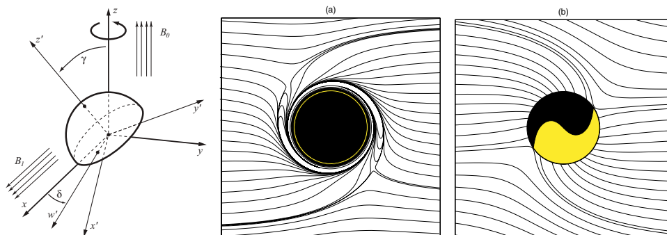
Figure 6. Lines of the magnetic field which is asymptotically uniform and perpendicular to the rotation axis. The equatorial plane is shown as viewed from top, i.e. along the rotation axis, (a) in the frame of zero angular momentum observers orbiting at constant radius; (b) in the frame of freely falling observers. In the panel (b), two regions of ingoing/outgoing lines are distinguished by different levels of shading of the horizon (the hole rotates counter-clockwise, a = M ).
