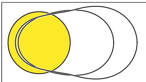
Figure 7. The cross-sectional area for the capture of magnetic field lines (asymptotically uniform magnetic field perpendicular to the rotation axis). The three curves correspond to different values of the black-hole angular momentum: a = 0 (the black hole cross-section is a perfect circle and its projection coincides with the black-hole horizon of radius 2M , indicated here by shading), a = 0.95M , and a = M (the most deformed shape refers to the maximally rotating case). Non-vanishing cross-sectional area for the extreme case demonstrates that the Meissner-type expulsion of the magnetic field does not operate on non-axisymmetric fields. The hole’s rotation axis is vertical and the magnetic field lines are pointing “towards us” (see Dovčiak et al. 2000 for details).
