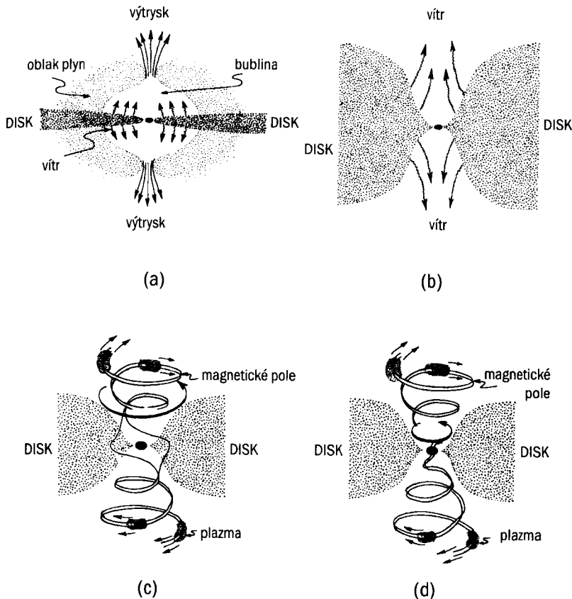
Figure 1. Four mechanisms of jet formation (drawing from “Černé díry a zborcený čas”, the Czech edition of “Black Holes and Time Warps”, by K. S. Thorne 2004).
