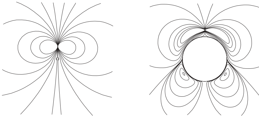
Figure 5. Field lines of the magnetic dipole placed far away from the extreme Reissner–Nordström black hole ( e = M , left panel), and close to the hole (right panel).
