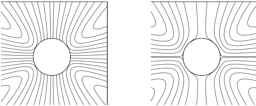
Figure 3. Field lines of the electric field induced by the “rotating geometry” of Kerr black hole in asymptotically uniform test magnetic field. a = 0.95M (left), and a = M (right).
