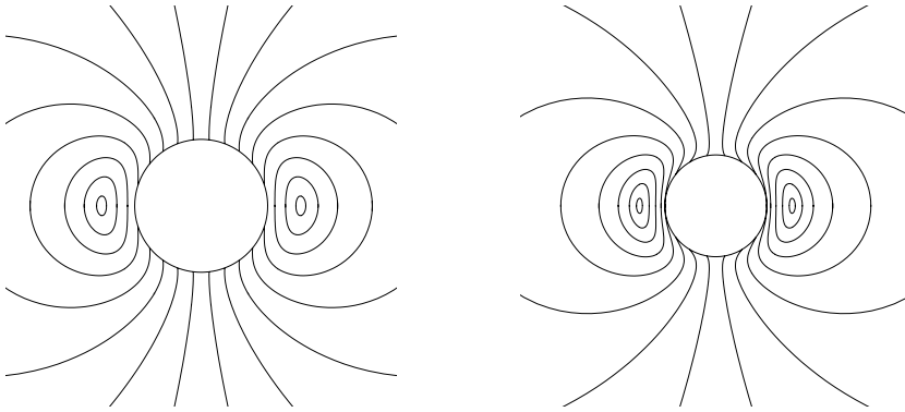
Figure 4. Field lines of the magnetic field of a current loop in the equatorial plane of Kerr black hole located at r = 1.5 r_+ . Two cases with a = 0.9M (left) and a = 0.995M (right) are shown.
