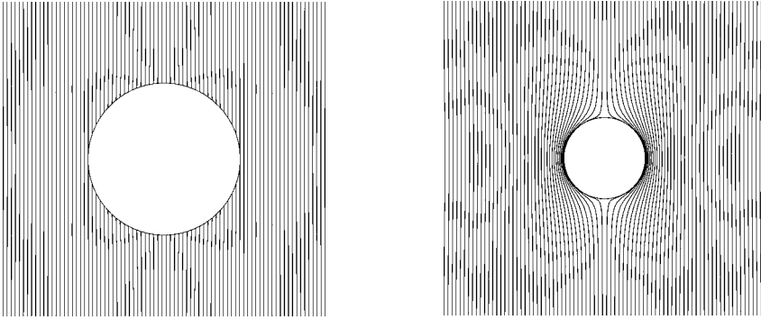
Figure 2. Field lines of the test magnetic field uniform at infinity and aligned with hole's rotation axis. Two cases with a = 0.5M (left) and a = M (right) are shown.
