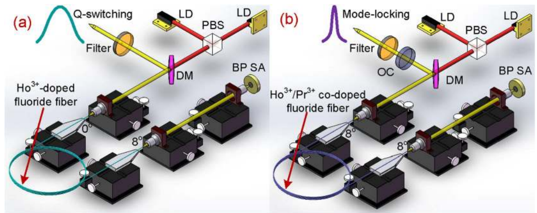
Figure 3. Experimental setup of pulsed fluoride fiber lasers based using BP SA. (a) Passively Q-switched Ho 3+ -doped fluoride fiber laser. (b) Passively mode-locked Ho 3+ /Pr 3+ co-doped fluoride fiber laser. LD is the laser diode, PBS is the polarized beam splitter, DM is the dichroic mirror, OC is the output coupler.
