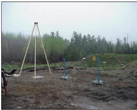
Fig. 4. The test specimen and the tripod holding the explosive charge.
