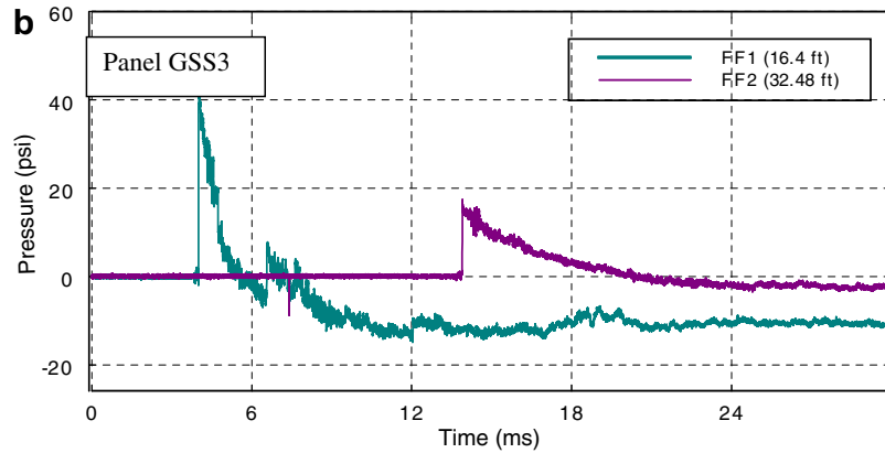
(a): Incident ( free field) pressure-time profiles
