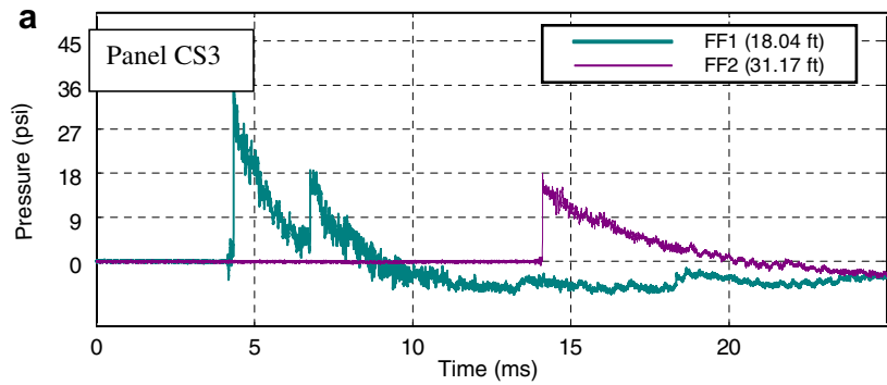
(a): Incident (free field ) pressure-time profiles
