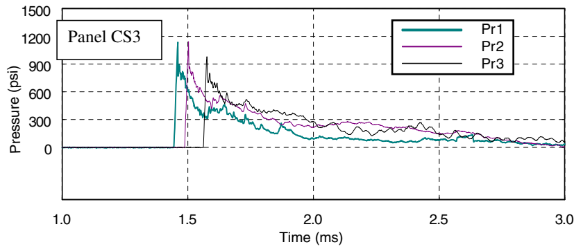
(b): Reflected pressure-time profiles
