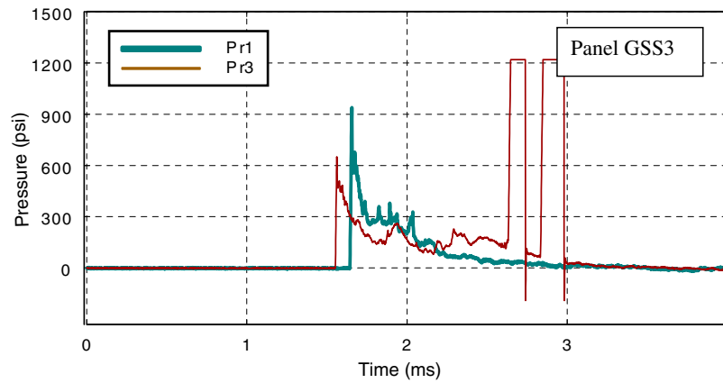
(b): Reflected pressure-time profiles
