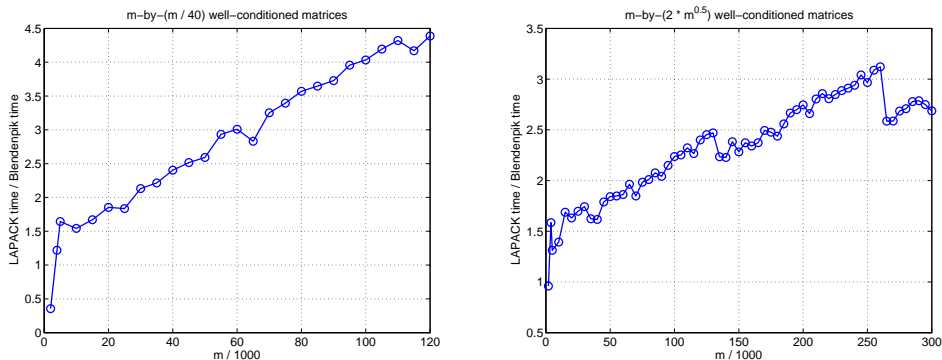
FIGURE 1.1. Comparison between LAPACK and the new solver for increasingly larger matrices. Graphs show the ratio of LAPACK’s running time to Blendenpik’s running time on random matrices with two kinds of aspect ratios.
