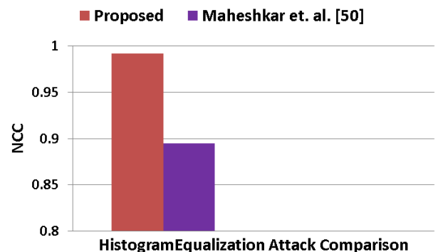
FIGURE 22. Comparison of average value of NC for four cover images for the proposed technique with the existing techniques under Histogram Equalization attack.
