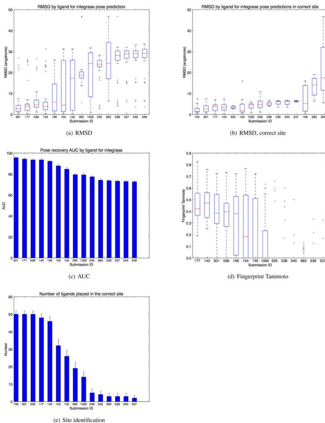
Fig. 4. Ranked performance on pose prediction, by various metrics. (a)-(b), box/whisker plots showing performance by ligand as judged by RMSD; (b) focuses only on the subset of ligands placed within the correct site. (c) shows performance judged by AUC, by ligand; and (d) shows performance by ligand as judged by interaction fingerprint Tanimoto scores. (e) shows the number of ligands placed into the correct binding site for each submission. For bar plots, normal submissions are shown in blue, while control models (300, 301) are shown in gray, as discussed in the text.
