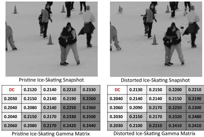
Fig. 11. Snapshots of the pristine and distorted Ice-Skating sequence, along with the computed \gamma matrices from corresponding frame-difference DCT coefficients. Notice how the \gamma values differ between the pristine and distorted sequences.
