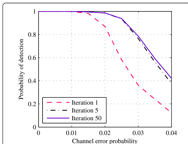
Figure 4 C(2,1,7): Probability of detection compared with P_e for L = 200 .
