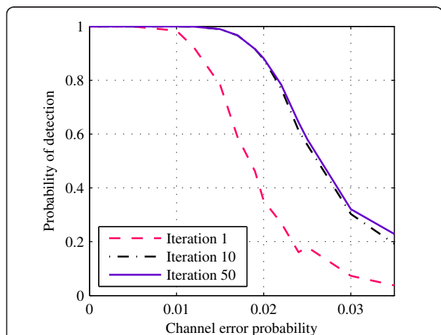
Figure 2 C(3,2,3): Probability of detection compared with P_e .
