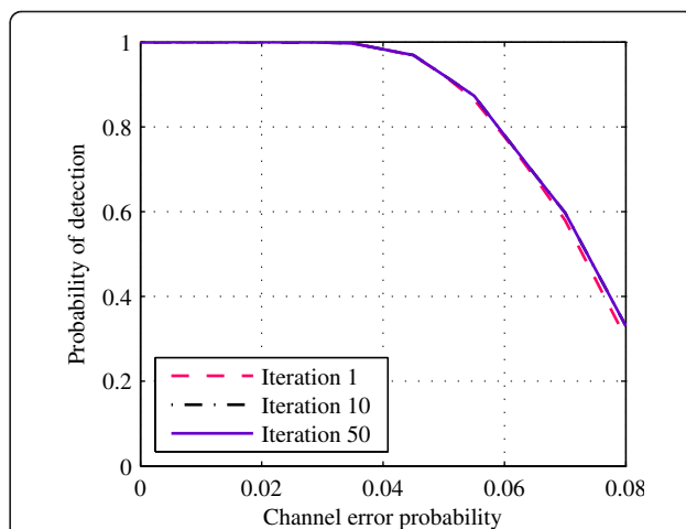
Figure 3 C(3,1,4): Probability of detection compared with P_e .
