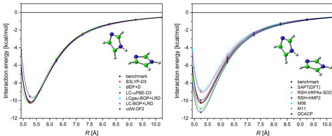
FIG. 7. Potential energy curves for the imidazole dimer. See Fig. 1 for explanations.
