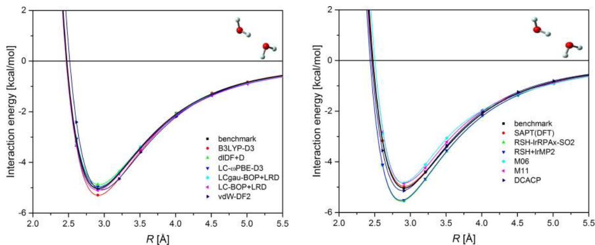
FIG. 1. Potential energy curves for the water dimer. The left panel compares the performance of DFT+D-type methods and of a functional with nonlocal correlation, whereas the right panel includes parametrized (hybrid) semilocal functionals and methods using virtual orbitals. Lines are drawn only to guide the eye.
