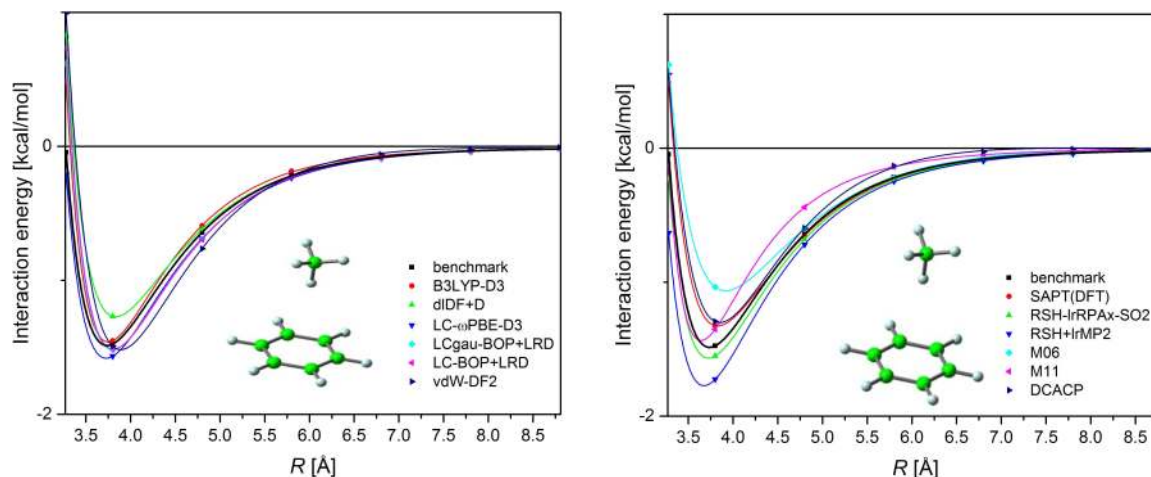
FIG. 5. Potential energy curves for the benzene-methane dimer. See Fig. 1 for explanations.
