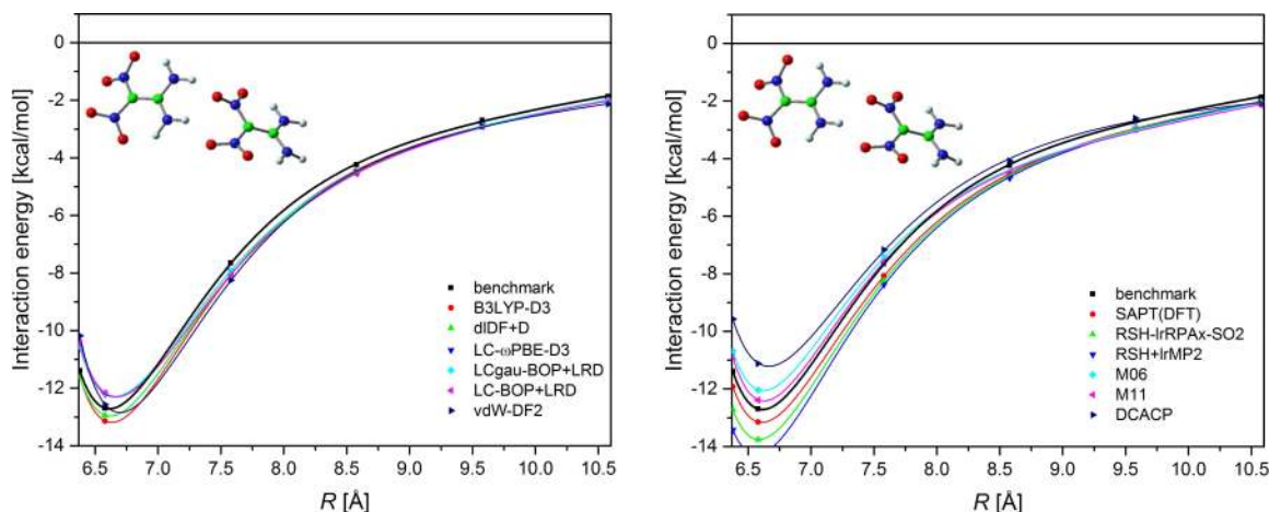
FIG. 9. Potential energy curves for the FOX-7 dimer. See Fig. 1 for explanations.
