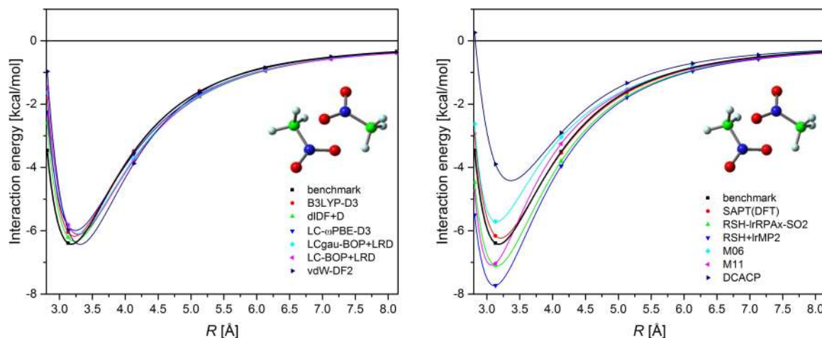
FIG. 3. Potential energy curves for the nitromethane dimer. See Fig. 1 for explanations.
