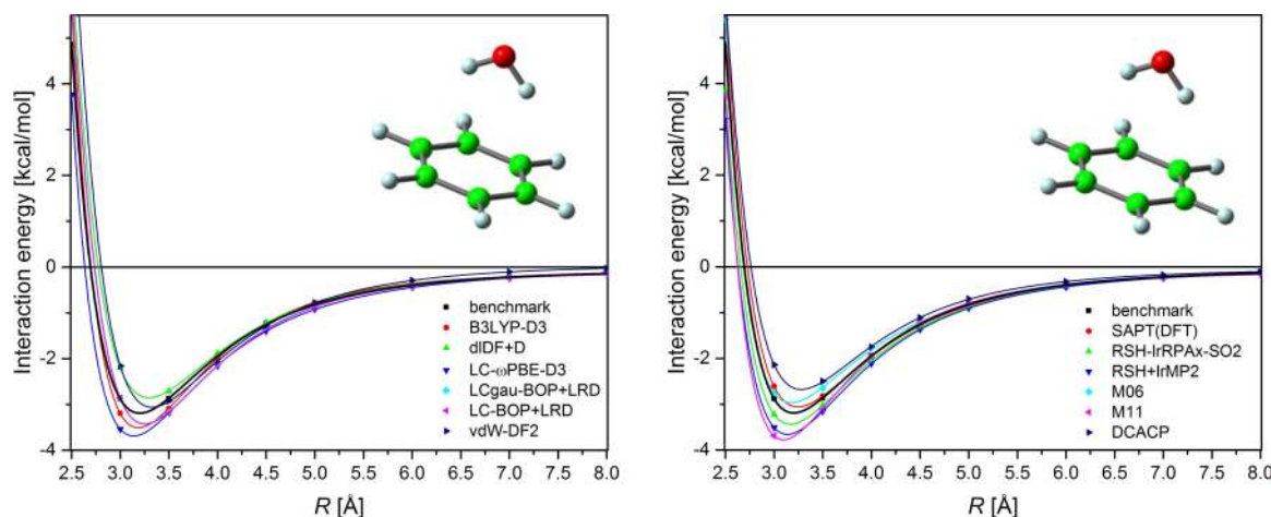
FIG. 6. Potential energy curves for the benzene-water dimer. See Fig. 1 for explanations.
