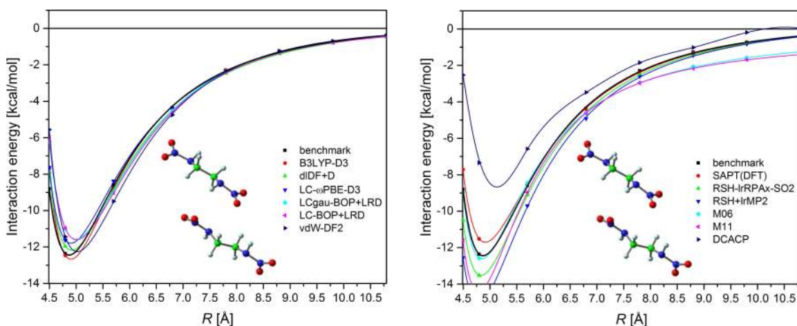
FIG. 10. Potential energy curves for the EDNA dimer. See Fig. 1 for explanations.
