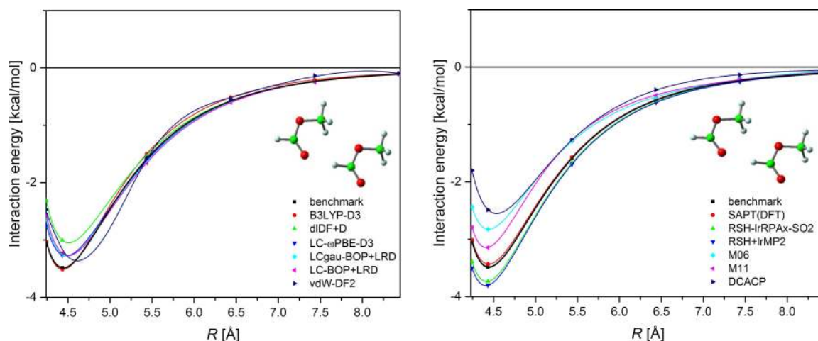
FIG. 4. Potential energy curves for the methylformate dimer. See Fig. 1 for explanations.
