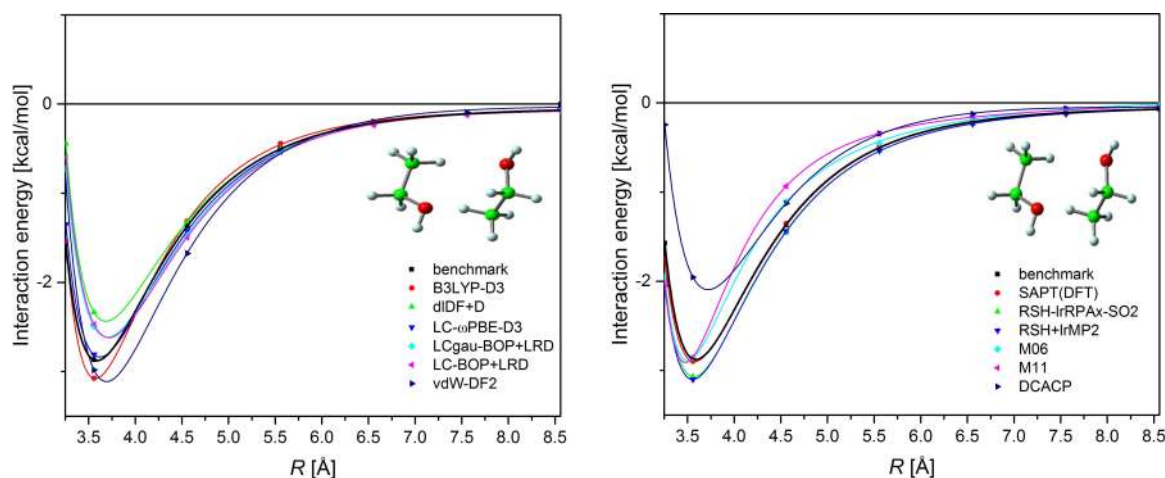
FIG. 2. Potential energy curves for the ethanol dimer. See Fig. 1 for explanations.
