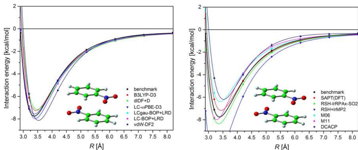
FIG. 8. Potential energy curves for the nitrobenzene dimer. See Fig. 1 for explanations.
