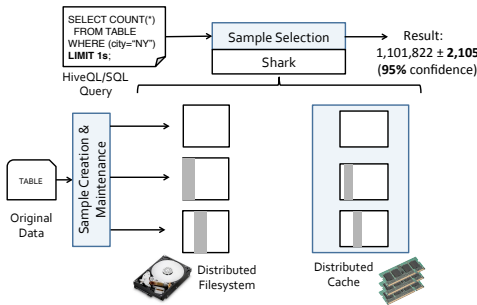
Figure 3. BlinkDB architecture.
