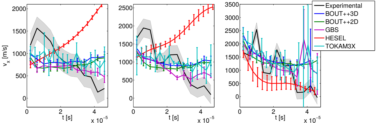
FIG. 8. Radial velocity of the blob as function of time for “case 1” (left), “case 2” (middle), and “case 3” (right), obtained from numerical simulations and experimental measurements (the gray shaded region represents the experimental uncertainty due to the finite spatial resolution of the probes).
