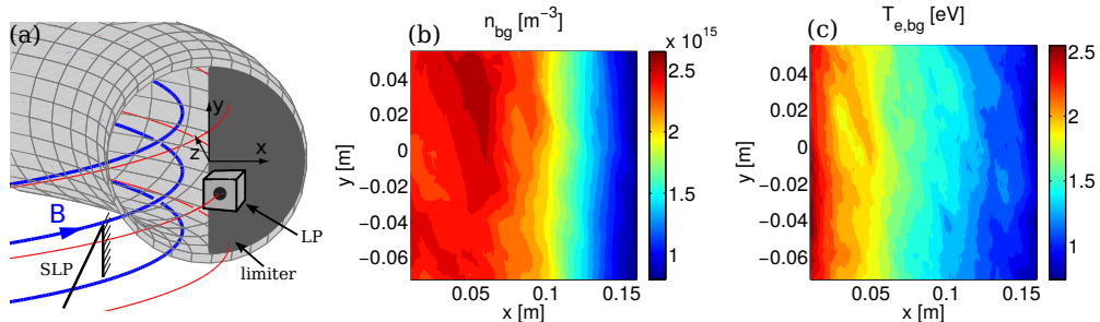
FIG. 1. (a) Schematic representation of the TORPEX experiment. The limiter located in the low-field side region is shown together with the probes used to perform blob conditional sampling. Note that SLP is not represented at 180^\circ from the limiter as it is in the experiment for drawing convenience. (b-c) Background profiles of n and T_e in the low-field side region, where blobs propagate. The profiles are measured in a poloidal plane 3 cm away from the limiter.
