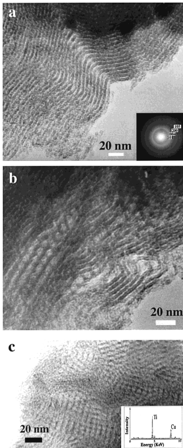
Figure 2. TEM micrographs of two-dimensional hexagonal mesoporous \text{TiO}_2 recorded along the (a) [110] and (b) [001] zone axes, respectively. Inset in part a is selected-area electron diffraction patterns obtained on the image area. (c) TEM image of cubic mesoporous \text{TiO}_2 accompanied by the corresponding (inset) EDX spectrum acquired for this sample.
